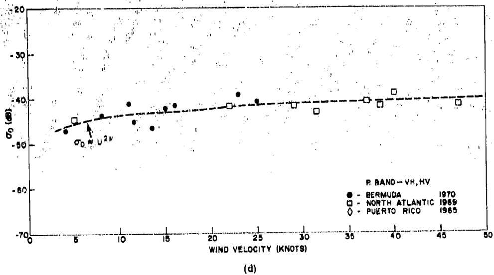
Fig. 8 (Continued) - Median NRCS of the sea vs wind velocity; cross-polarization upwind, 30° depression angle
