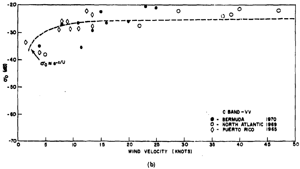
Fig. 4 - Median NRCS of the sea vs wind velocity; X and C bands upwind, 30° depression angle
