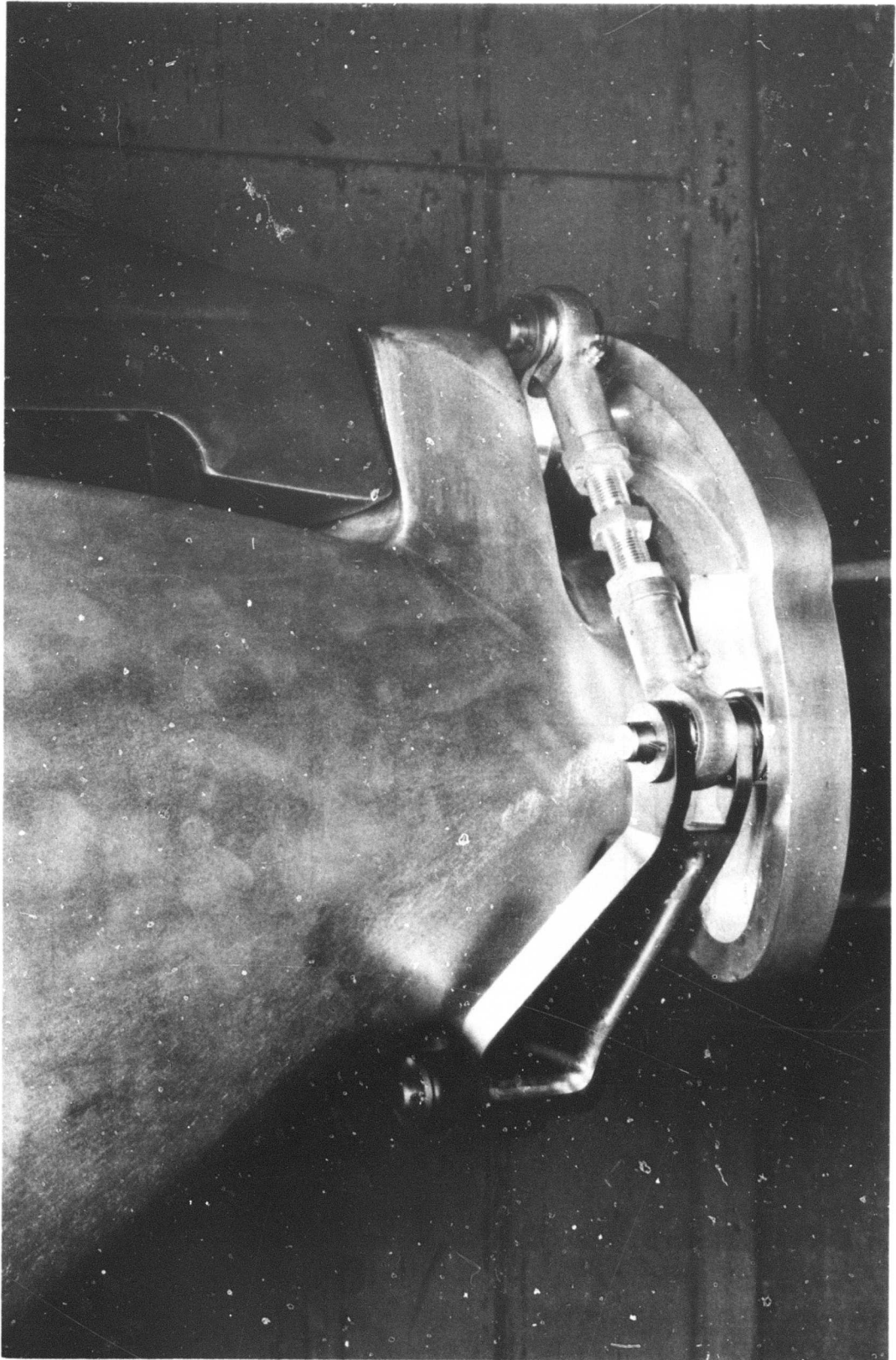
Figure 3. Blade Flap Actuation Mechanism
