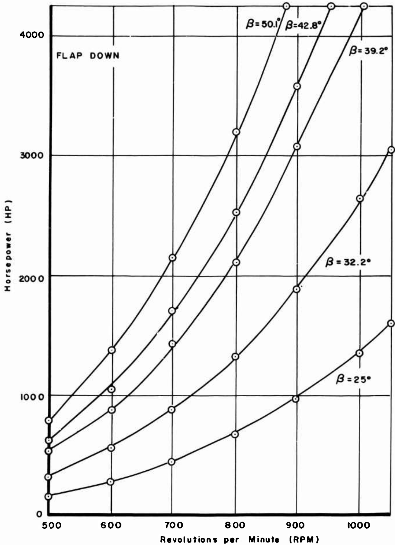
Figure 8. Horsepower vs Propeller Speed at Various Blade Angles - Full Blade Flap Deflection
