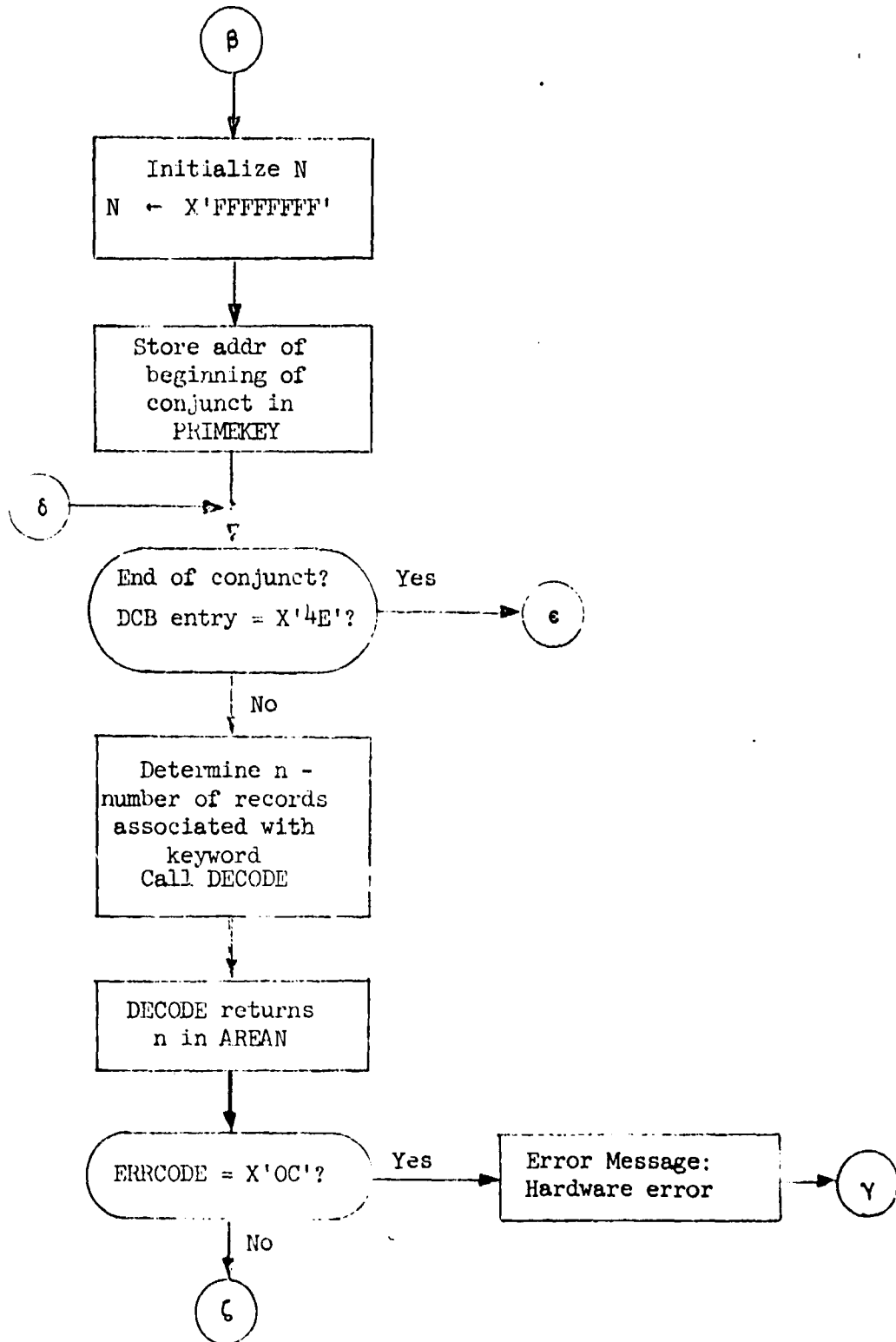
Figure B.4.c: Prime Keyword Selection
