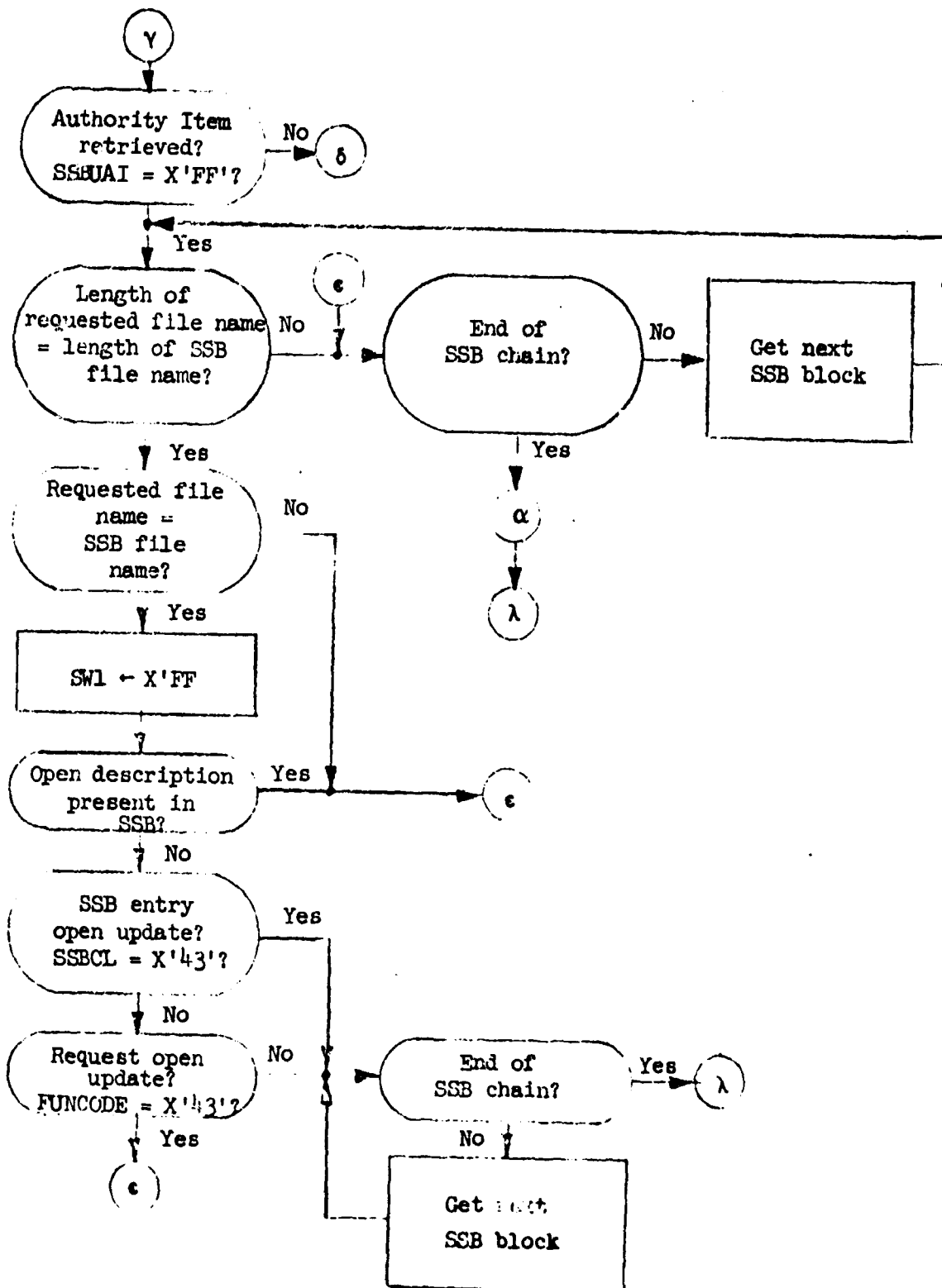
Figure B.1.e: SSB Check
