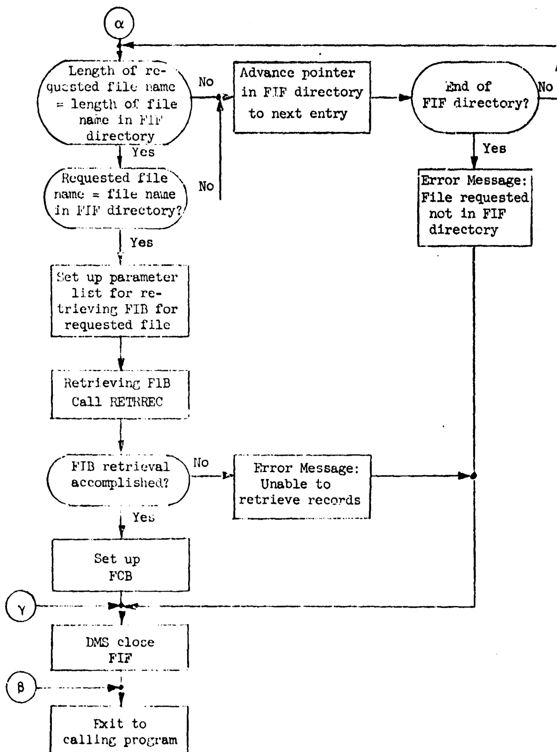
Figure B.2.b: Retrieval of File FIB and FCB
