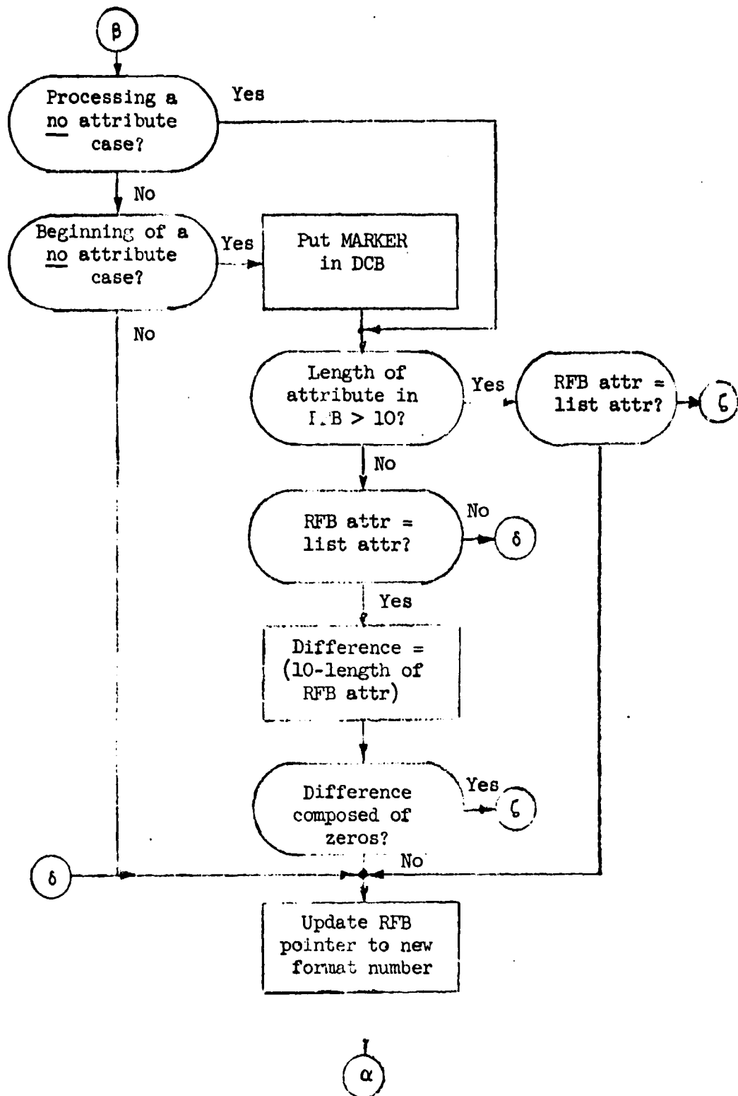
Figure B.5.c: Processing No Attribute Case
