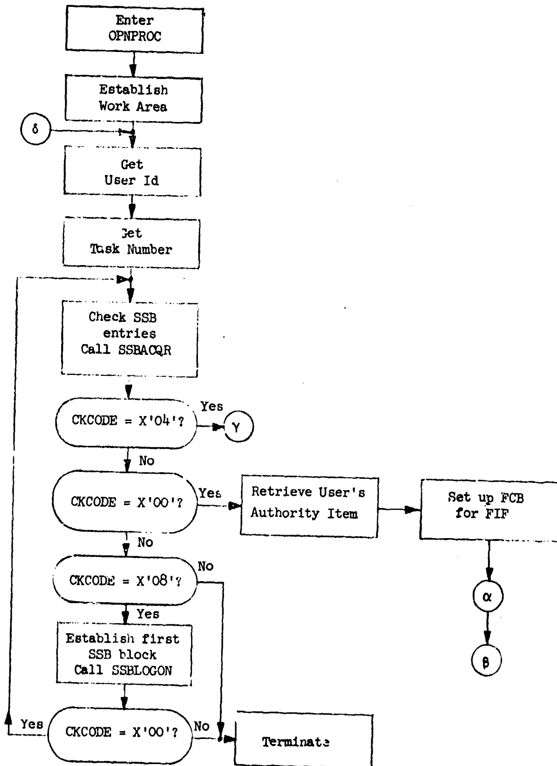
Figure B.1.a: OPNPROC Initialization. Retrieve SSB Chain.
