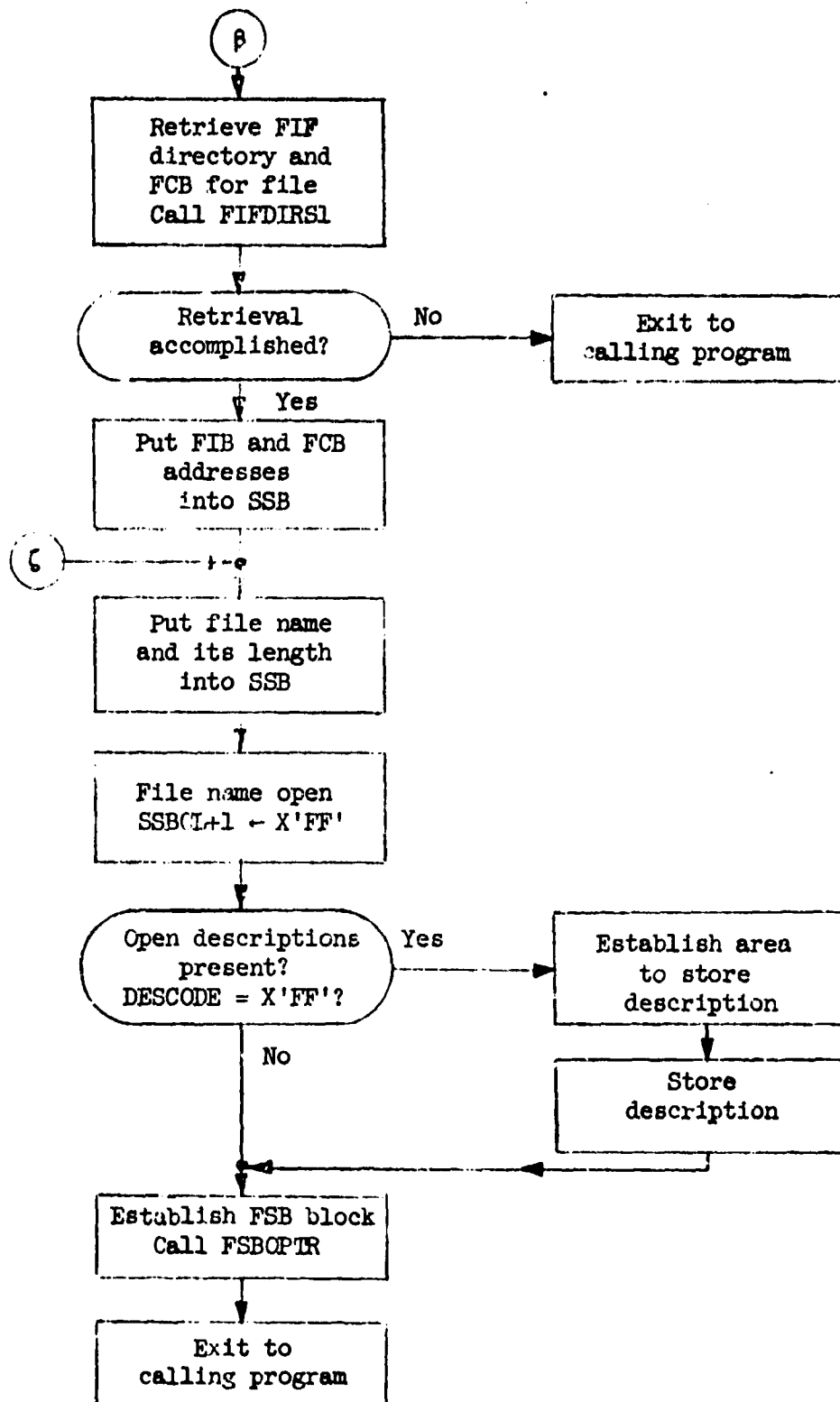
Figure B.1.c: Set up SSB. Establish FSB.
