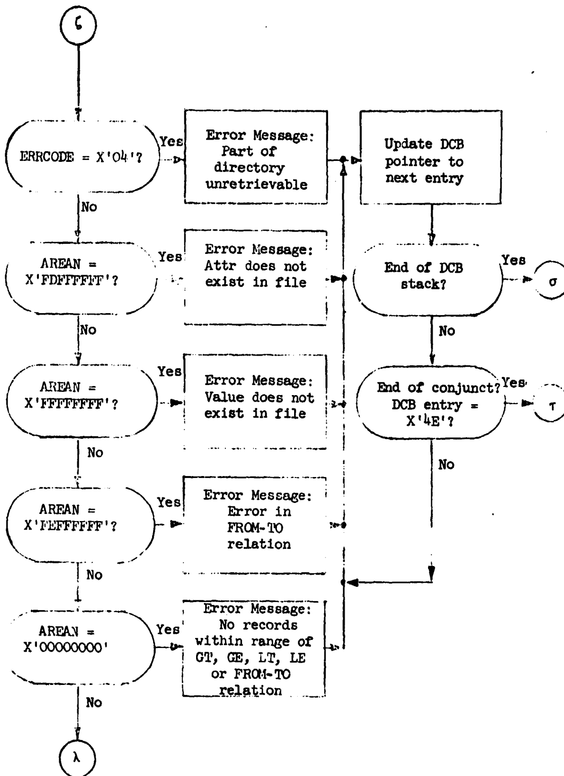
Figure B.4.d: Prime Keyword Selection
