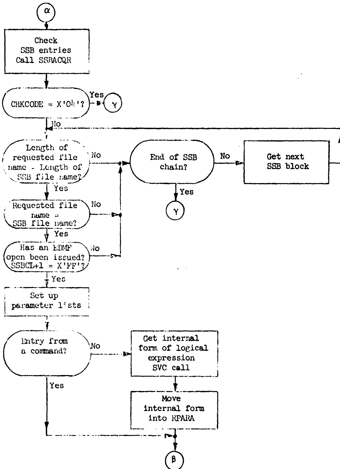
Figure B.3.b: SSB Check and Translation of Logical Expression
