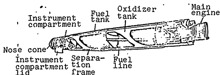
Structural schematic of an intermediate-range liquid fuel rocket.
