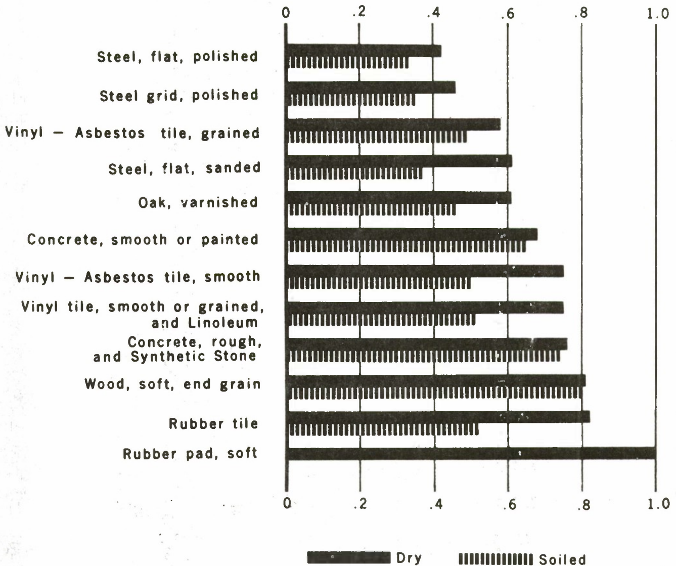
Figure 13. Mean coefficients of static friction of floor materials under eight shoe materials
