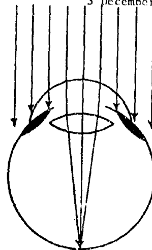
LONG ULTRAVIOLET AND VISIBLE
