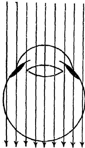
GAMMA AND X RADIATION
