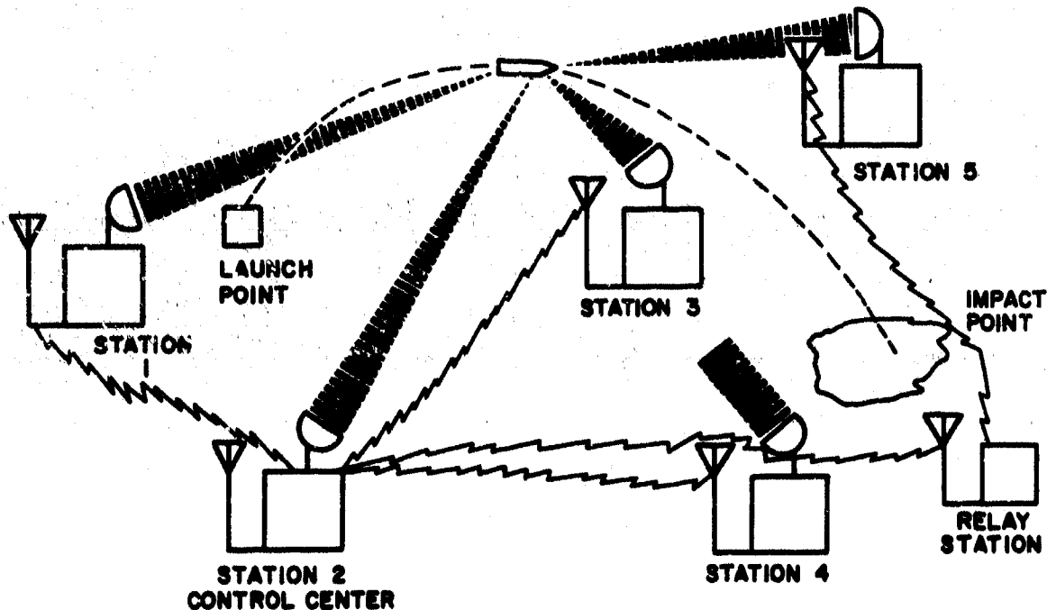
Figure 2. Method of Radar Chain Tracking of Missiles.
