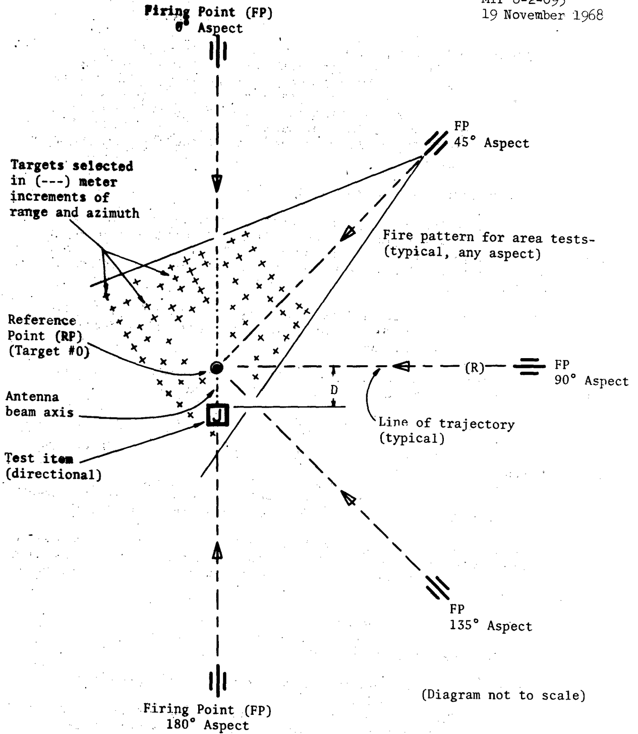
Figure 1. Test Setup for Ground-based Test Items.
