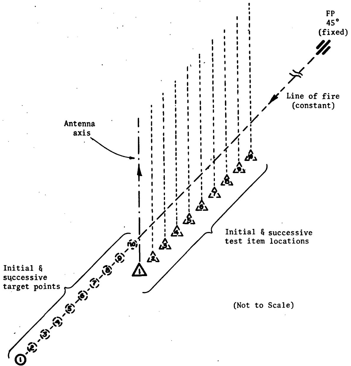
Figure 2. Test Setup for Angle-of-Fall Effect.
