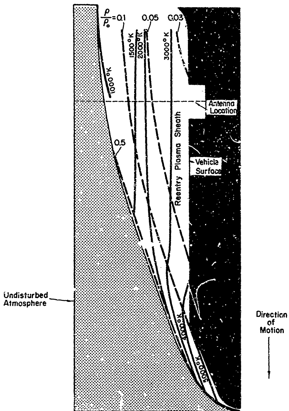
Figure 11 - 2 Plasma sheath surrounding a typical blunt - nosed ICBM reentry vehicle at 27 km ( Jackman et al. 1964, Figure 1).
