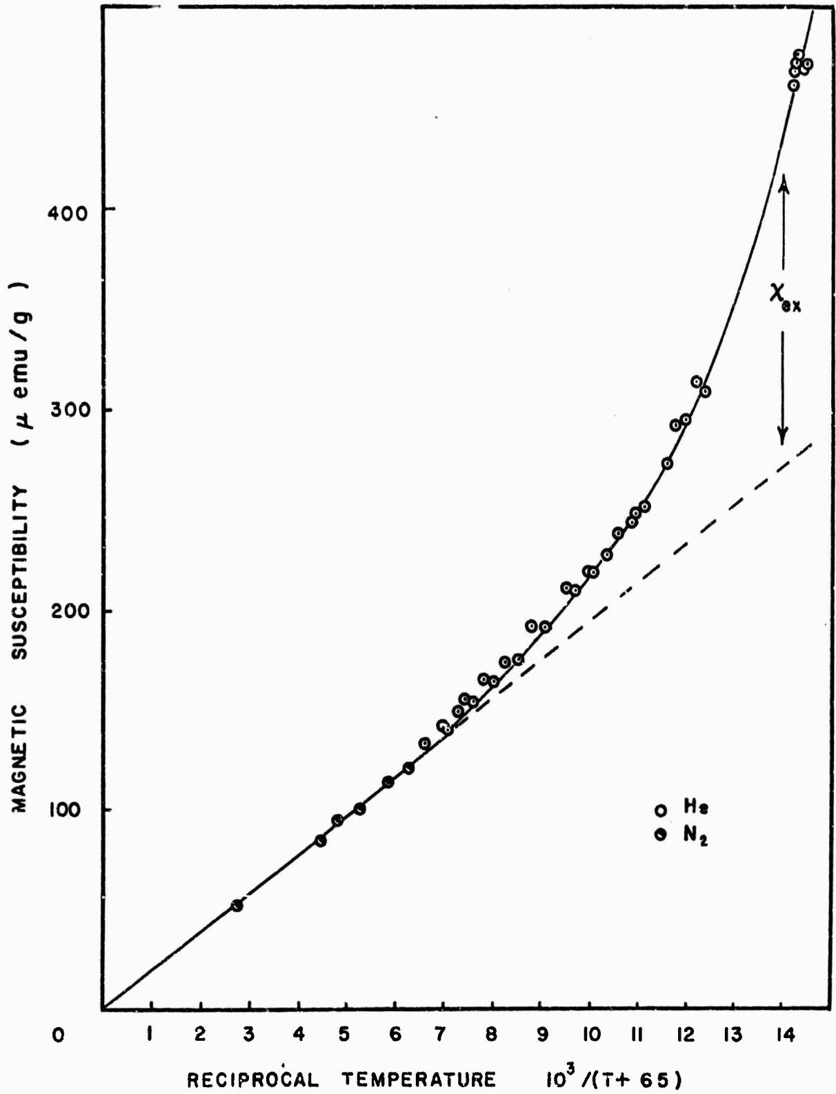
FIGURE 4. MAGNETIC SUSCEPTIBILITY OF ORTHORHOMBIC \text{YbMnO}_3 AS A FUNCTION OF (T+65)^{-1} OVER THE TEMPERATURE RANGE OF 4.2 - 322K
