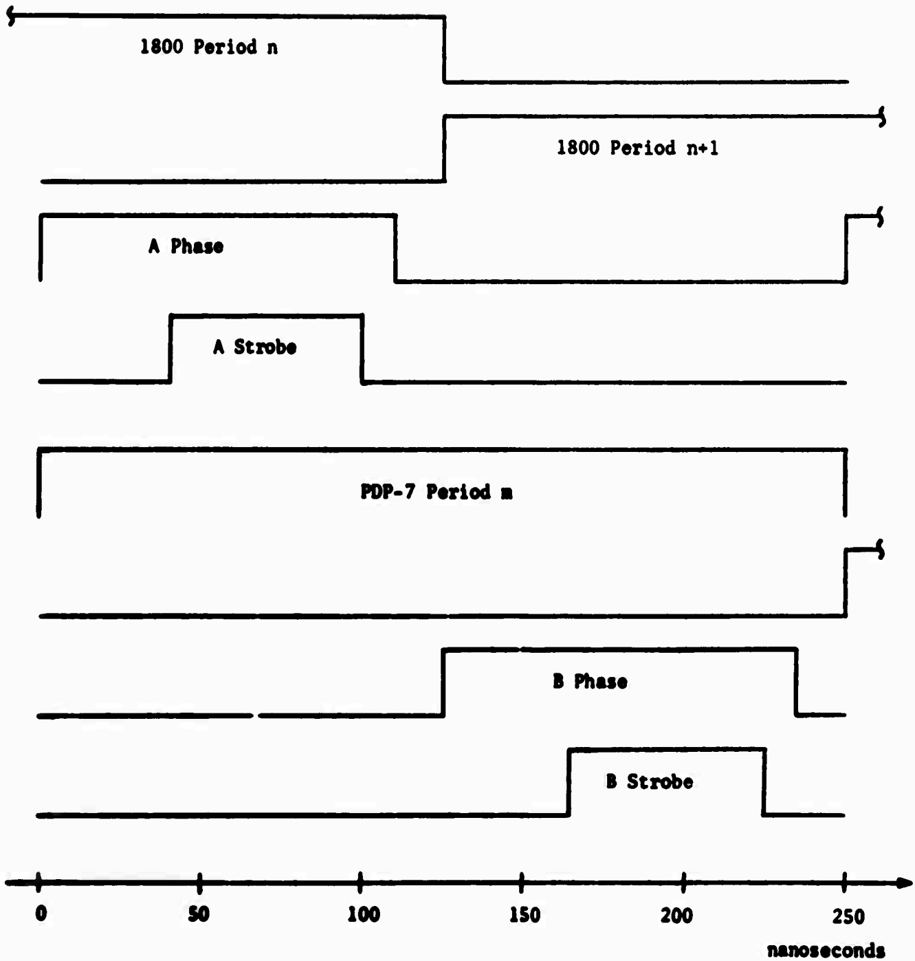
Figure 3.1: Schematic representation of Period, Phase, and Strobe timing relationships
