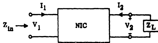
FIG. 1: NIC with load.
