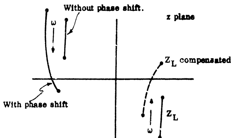
FIG. 21: Effect of phase shift on NIC performance.
