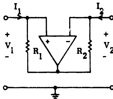
FIG. 16: Operational amplifier NIC.
