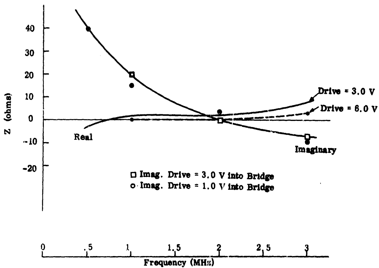
FIG. 14: Measured impedance of RL realization.
