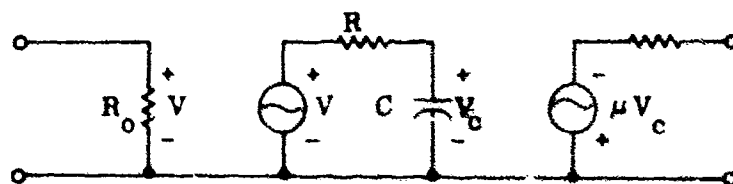
FIG. 20: Amplifier model with phase shift.
