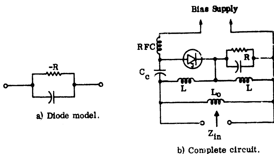
FIG. 22: Tunnel-diode negative-reactance circuit.
