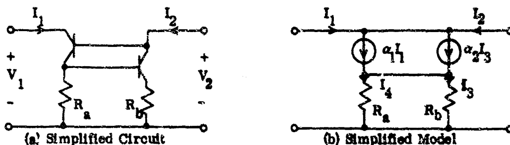
FIG. 2: Yanagisawa NIC.
