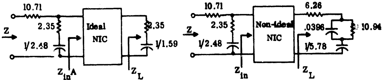
FIG. 9: Load realization with ideal and non-ideal NIC's.
