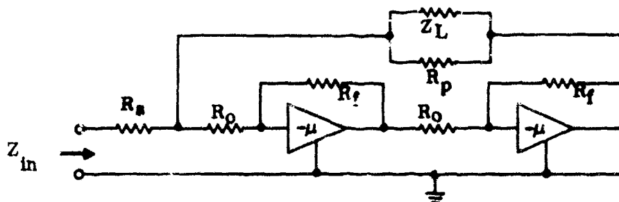
FIG. 19: Feedback amplifier NIC with compensation.
