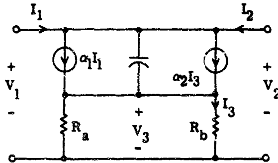
FIG. 3: High-frequency model of NIC.
