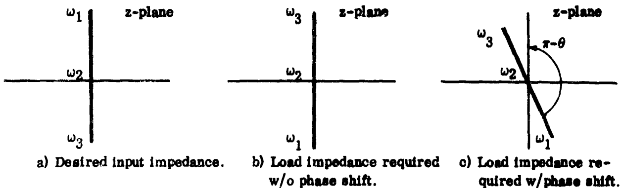
FIG. 5: Effect of phase shift in NIC.
