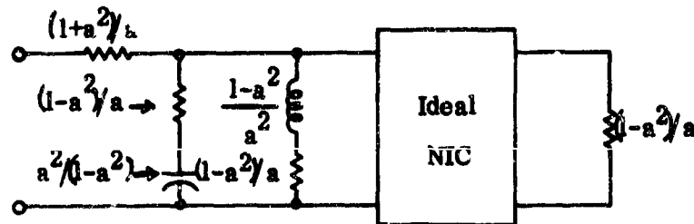
FIG. 12: Alternate realization of Z(s) .
