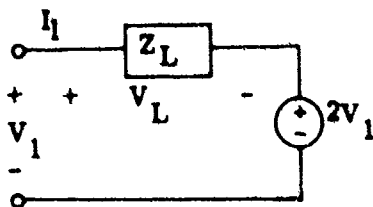
FIG. 17: Amplifier NIC .
