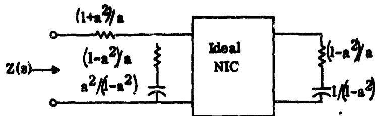
FIG. 6: RC realization of desired load.
