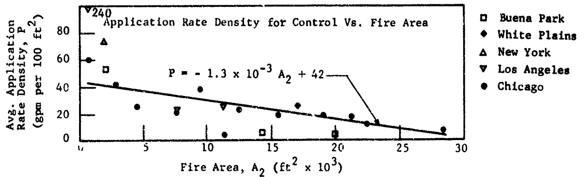
Fig. 3 WATER APPLICATION AND TIME USED TO CONTROL NONRESIDENTIAL FIRES (Average Within Each Class)
