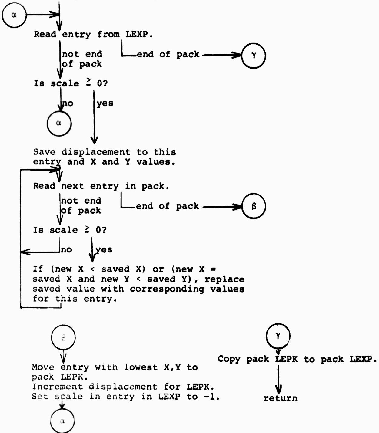
Figure 11. Subroutine EXORD
