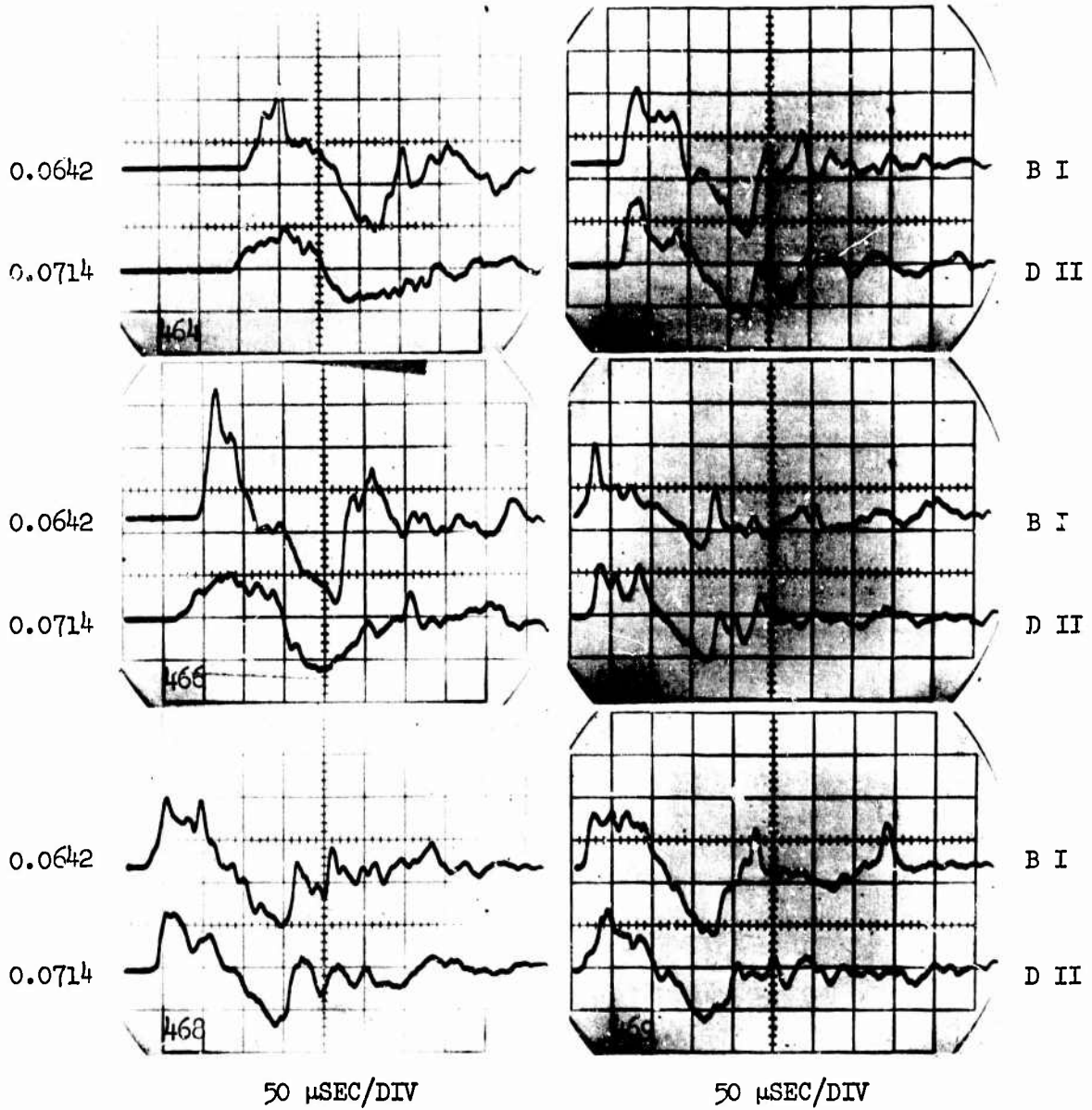
Figure A49 Boom signatures for group 344 -- 0.22 caliber projectiles, M = 3.0, high-speed nozzle no. 1, and 24 inch inlet.
