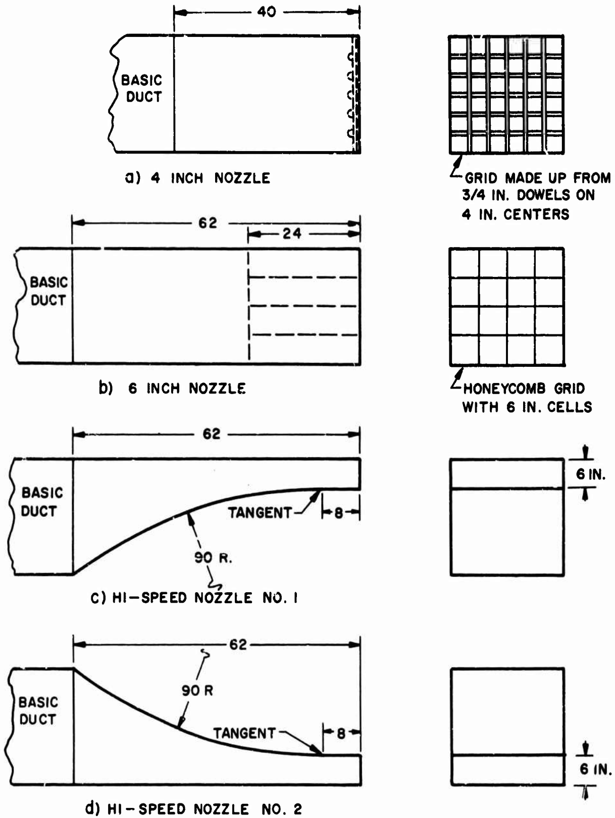
Figure 6 Duct extensions used in the task II program.
