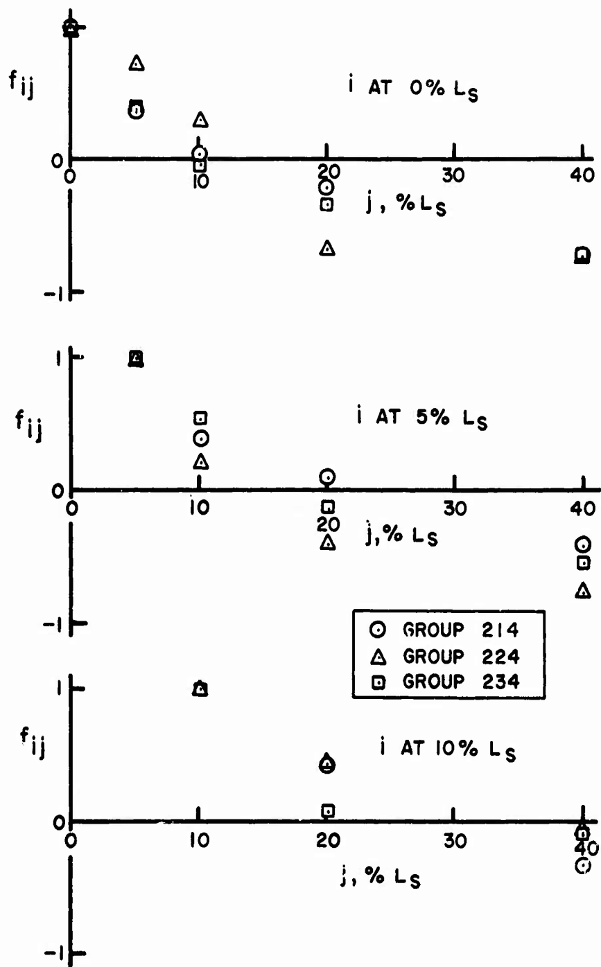
Figure 30 Experimental values of boom signature two-point correlation coefficients. M = 2.55 , B projectile, L_s = 9.01 inches, blower inlet diameter = 24 inches.
