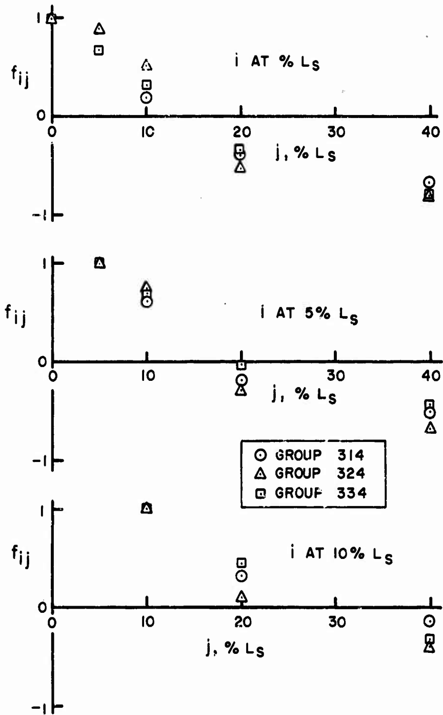
Figure 31 Experimental values of boom signature two-point correlation coefficients. M = 3.0 , L_s = 6.41 inches, 0.22 caliber bullet, blower inlet diameter = 24 inches.
