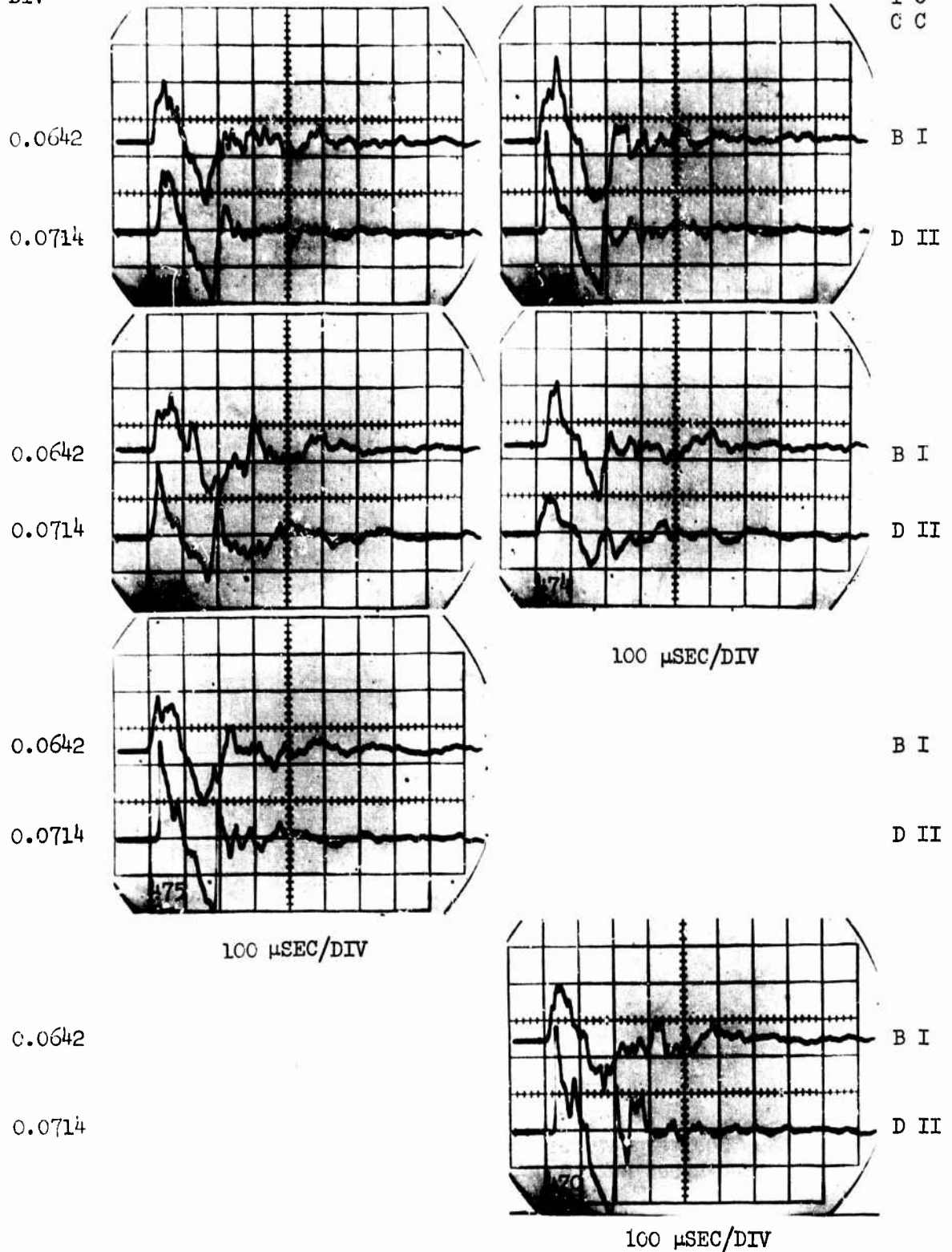
Figure A50 Boom signatures for group 344 -- 0.22 caliber projectiles; M = 3.0, high-speed nozzle no. 1, and 24 inch inlet.
