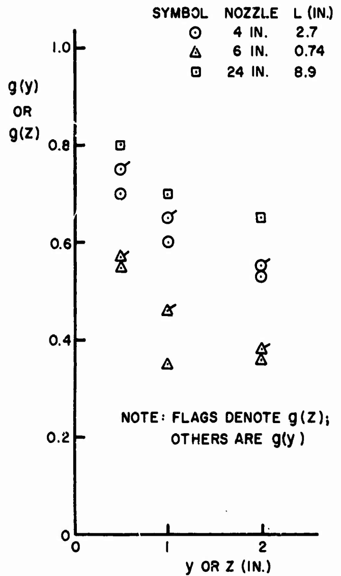
Figure 17 Two-point transverse correlation coefficients determined by direct measurements.
