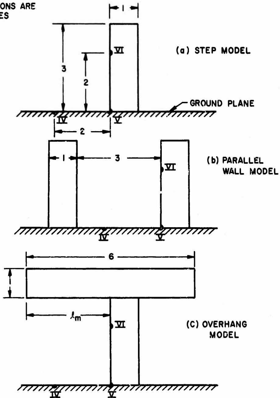
Figure 3 Two-dimensional topographical models as viewed looking in the +z direction.
