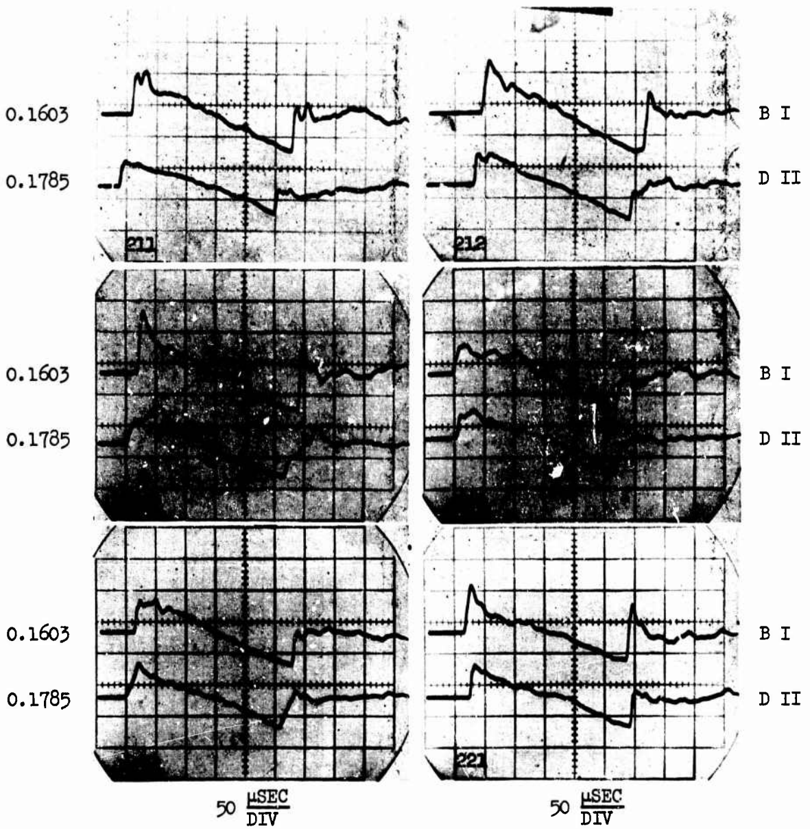
Figure A17 Boom signatures for group 215 -- B projectiles, M = 2.56, 4 inch nozzle, and open inlet.
