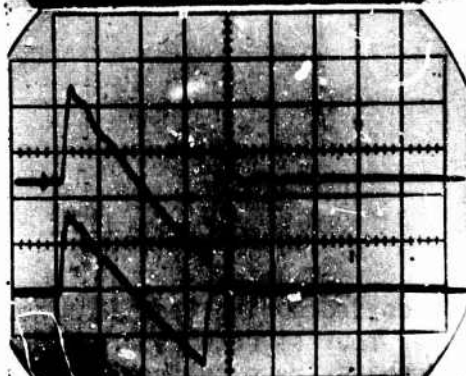
Figure A5 Basic signatures recorded during tasks II and IV using 0.22 caliber projectiles at M = 3.0.
