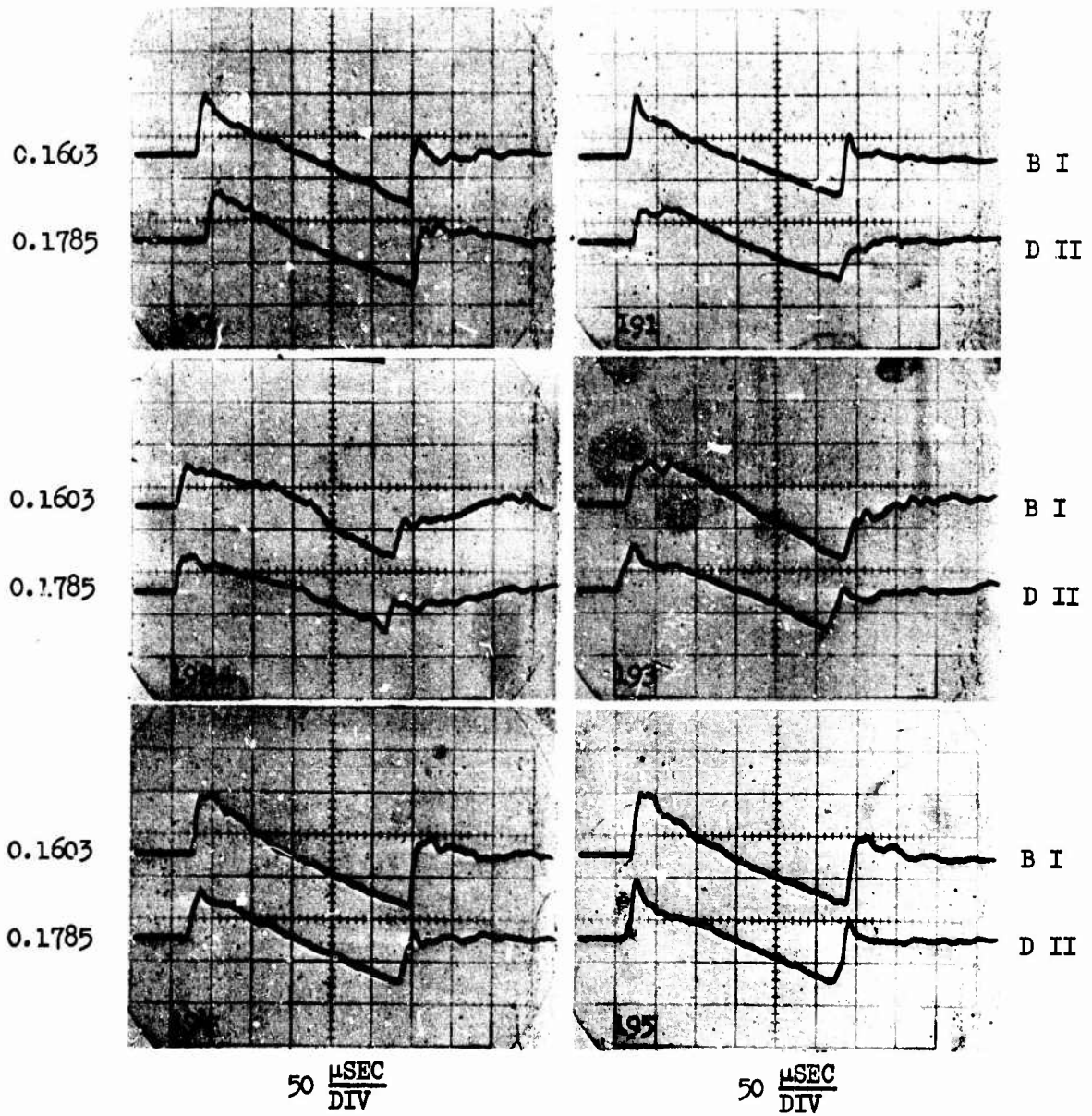
Figure A15 Boom signatures for group 214 -- B projectiles, M = 2.56, 4 in. nozzle, and 24 in. inlet.
