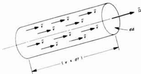
Fig. 2.2. Particle Flow Concept of Current. The particles contained within the volume element will all exit through the differential area dA within dt if \bar{v} = v\bar{\Omega} .
