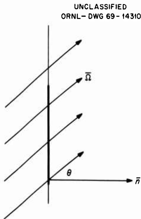
Fig. 2.5. Orientation of \bar{\Omega} -Directed Particles with Respect to a Unit Area Normal to the Direction Vector \vec{n} .
