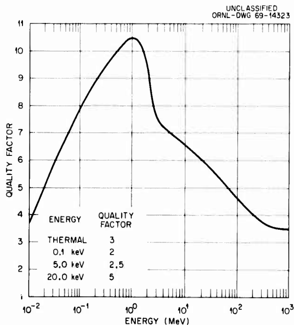
Fig. 2.19. Quality Factors for Neutrons. (From ref. 46.)
