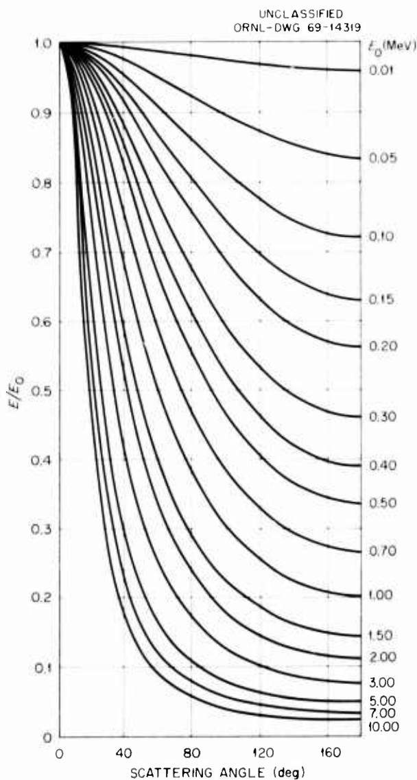
Fig. 2.14. Reduction in Gamma-Ray Energy by Compton Scattering. ( E_0 = initial energy; E = reduced energy.)
