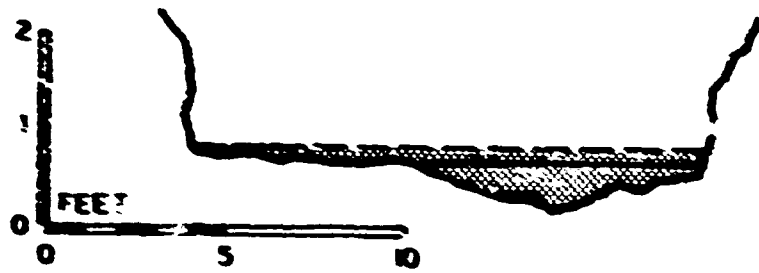
FIGURE 10. PROFILE OF THE SANK MUERTO CHANNEL 18
