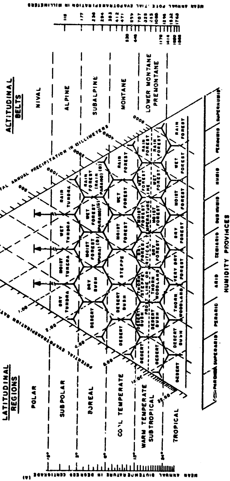
FIGURE 3. CLASSIFICATION OF WORLD LIFE ZONES BY L. R. HOLDRIDGE
