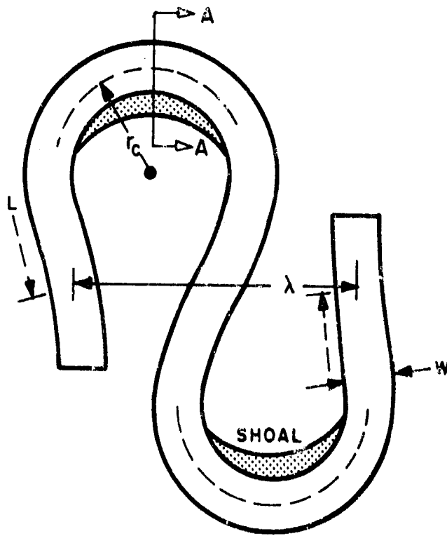
FIGURE 23. DEFINITION OF TERMS RELATING TO A RIVER MEANDER 10
