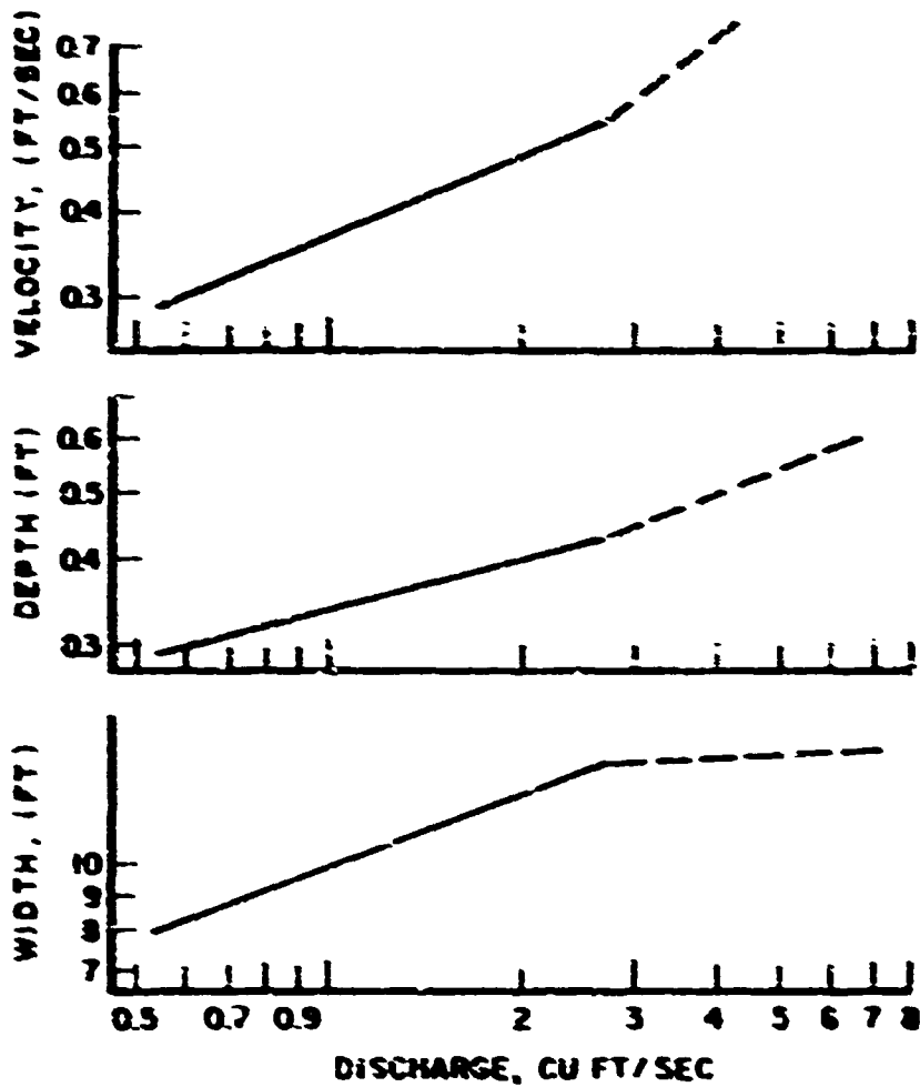
FIGURE 11. REGRESSION PLOTS OF FIELD DATA TAKEN AT SANK MUERTO STATION 18 (DOTTED LINE IS FOR BED-FULL CONDITION)
