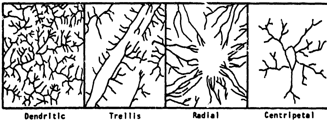
FIGURE 2. DRAINAGE PATTERNS OF RIVERS
