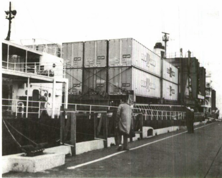
Figure 27. Tiedowns on Aft-Deck-Loaded Containers.
