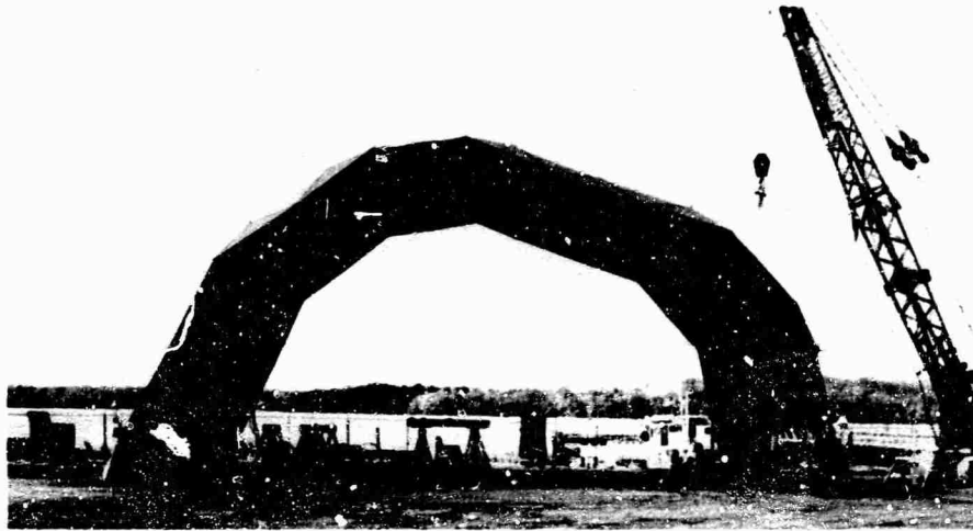
Fig. 25. Structure 85 percent complete – end view.
