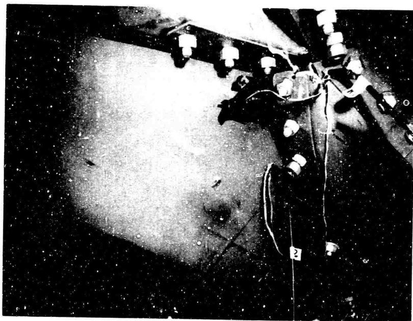
Fig. 74. Nodal point failure on side opposite load.
