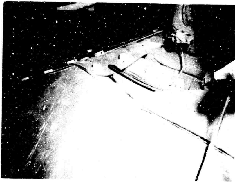
Fig. 73. Failure adjacent to nodal point on load side of beam.
