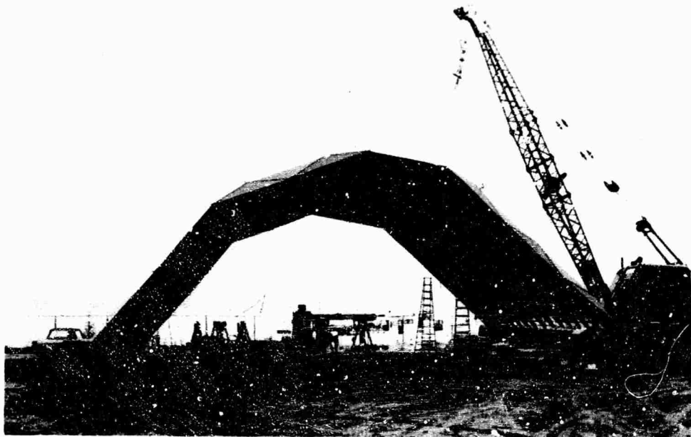
Fig. 20. Crane lift of structure at 60-percent completion.
