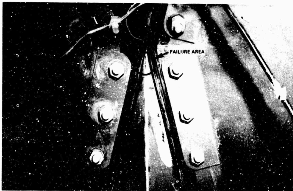
Fig. 82. Crack in parent material along panel fold line propagating from obtuse angle end of panel.
