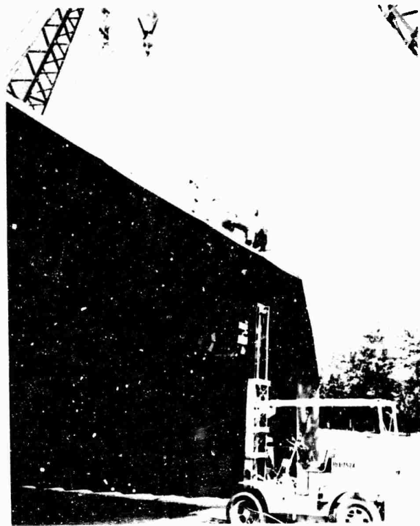
Fig. 42. Installation of bolts for joining of roof to sidewall.
