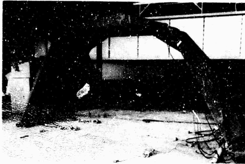
Fig. 68. Curved beam (without stiffeners) test setup.
