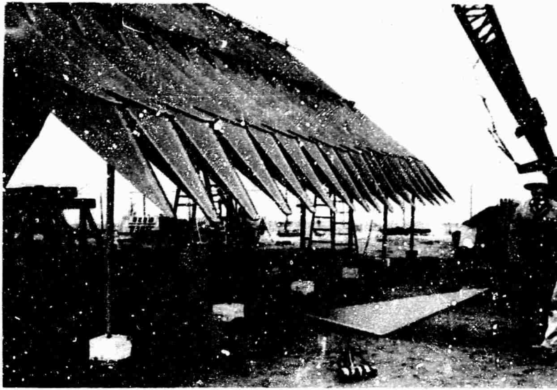
Fig. 23. Structure erection – 70 percent complete.
