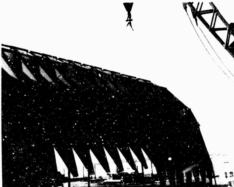
Fig. 24. Structure erection – 85 percent complete.
