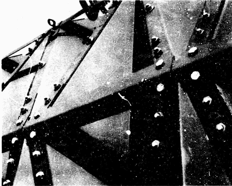
Fig. 46. Six-hole transverse stiffener installation.
