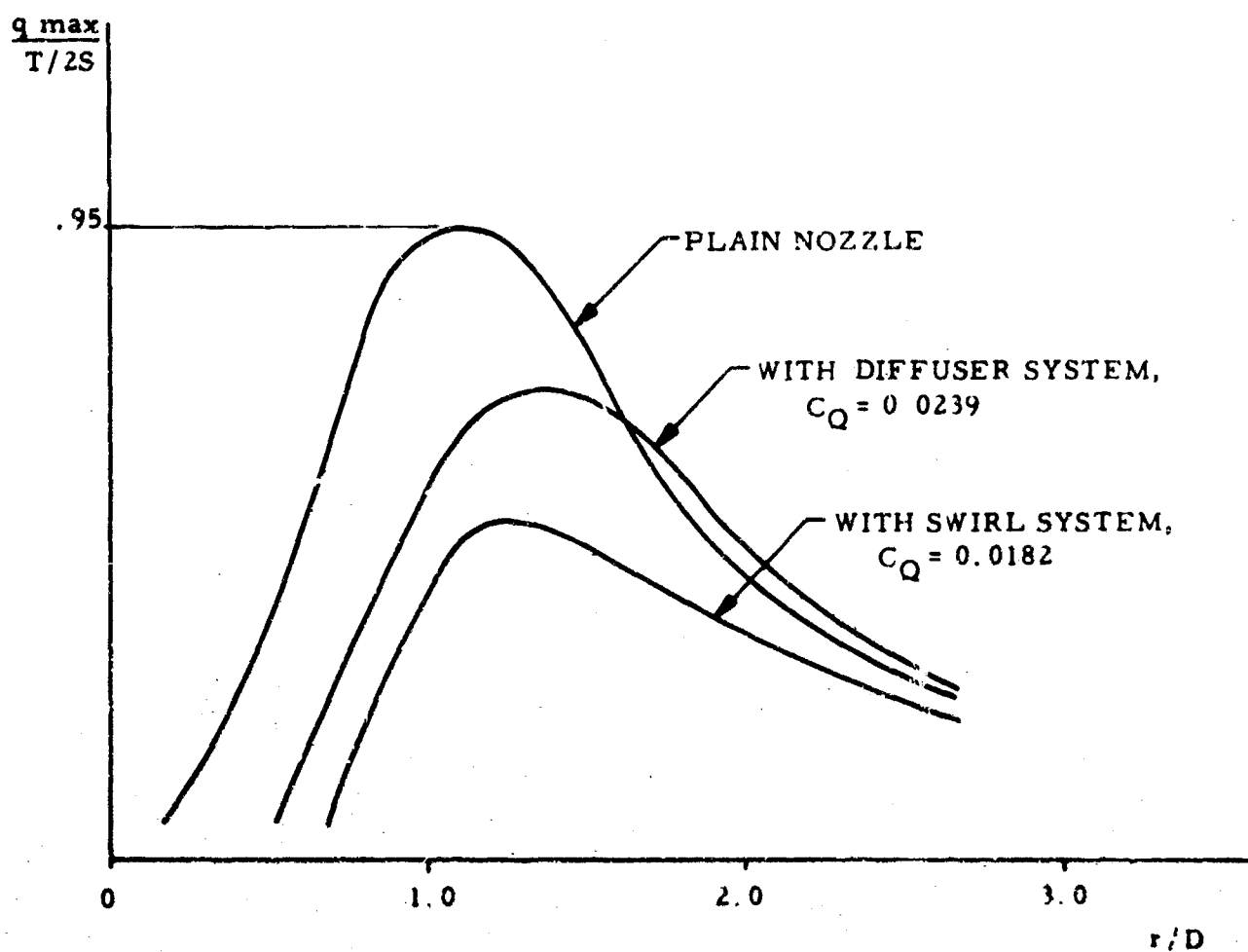
Figure 6. Variation of Maximum Ground Dynamic Pressure With Nozzle Configuration. ( h/D = 1.5 )
