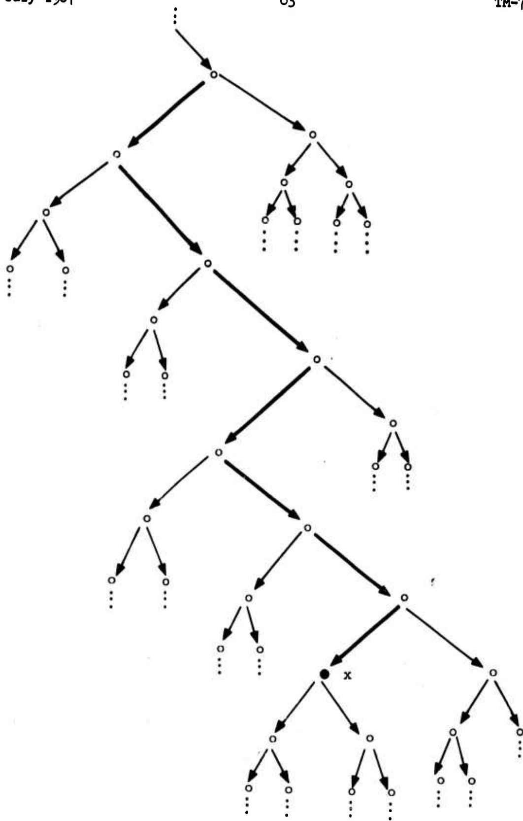
Figure 3. Diagram of an Ungenerated K -Algebra.
