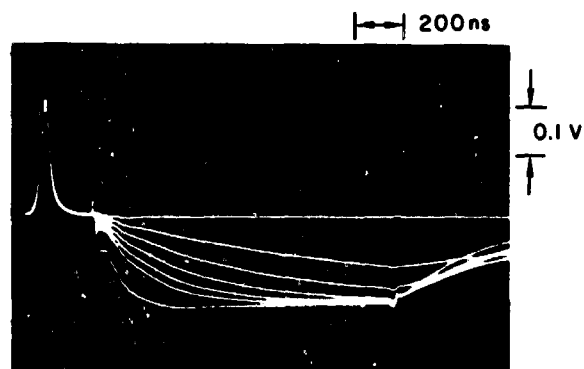
FIGURE 15 "TURN-ON" PULSE WITH VARYING RISE TIMES
