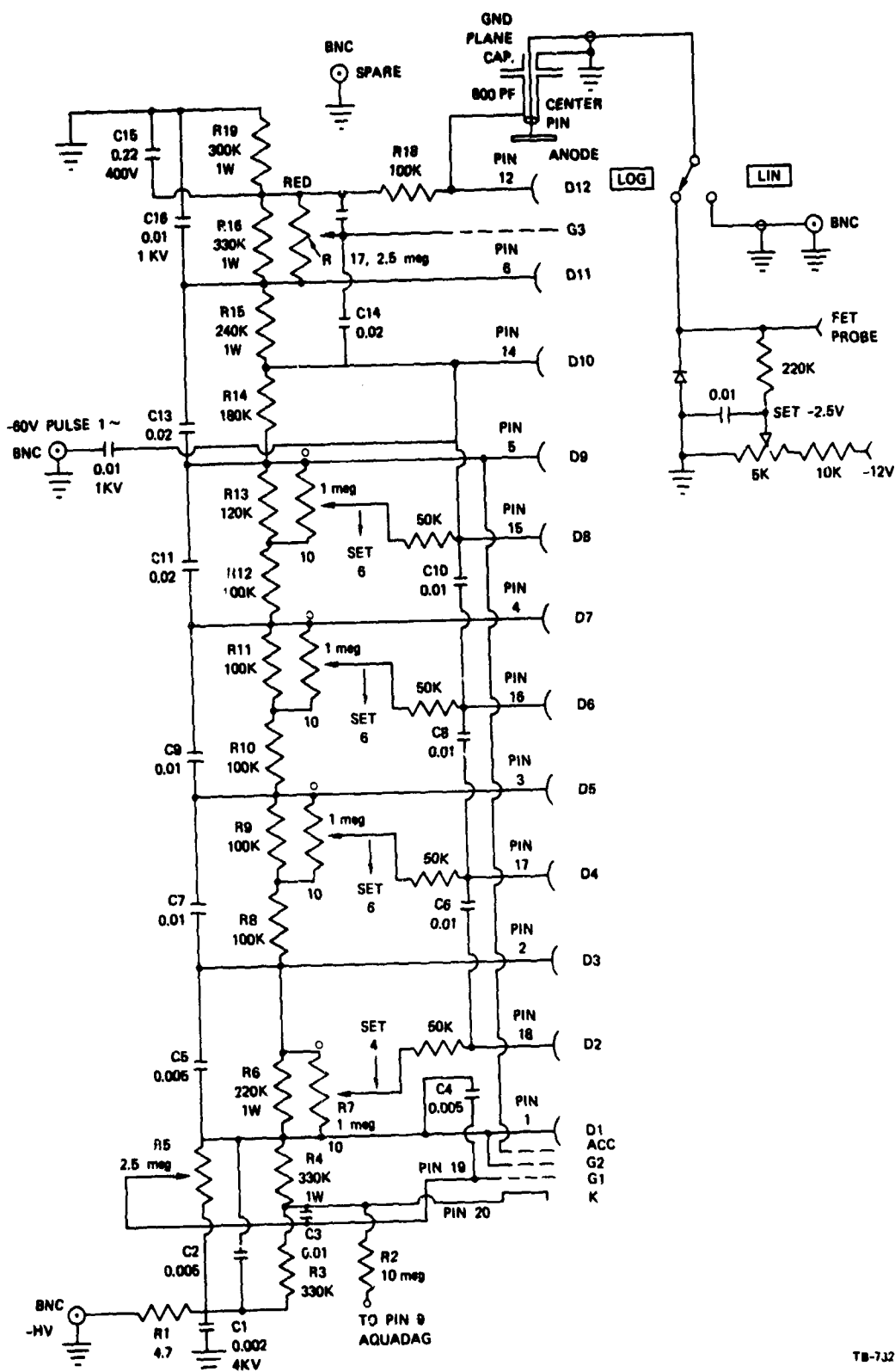
FIGURE 11 PHOTOMULTIPLIER TUBE WIRING DIAGRAM
