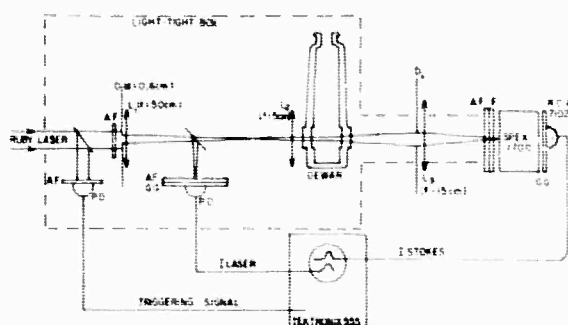
FIG. 4. Diagram of apparatus used for Raman intensity measurements. Explanation of symbols: D - diaphragm, A, F - attenuating filter, G, G - ground glass, P. D. - E. G. & G photodiode (SGD-100), L - lens, F - filter.
