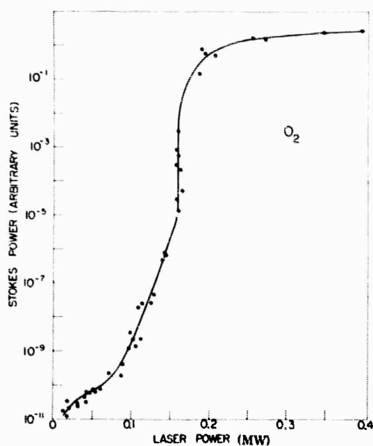
FIG. 5. Experimental curve for liquid oxygen showing Raman Stokes power as a function of incident ruby laser power.
