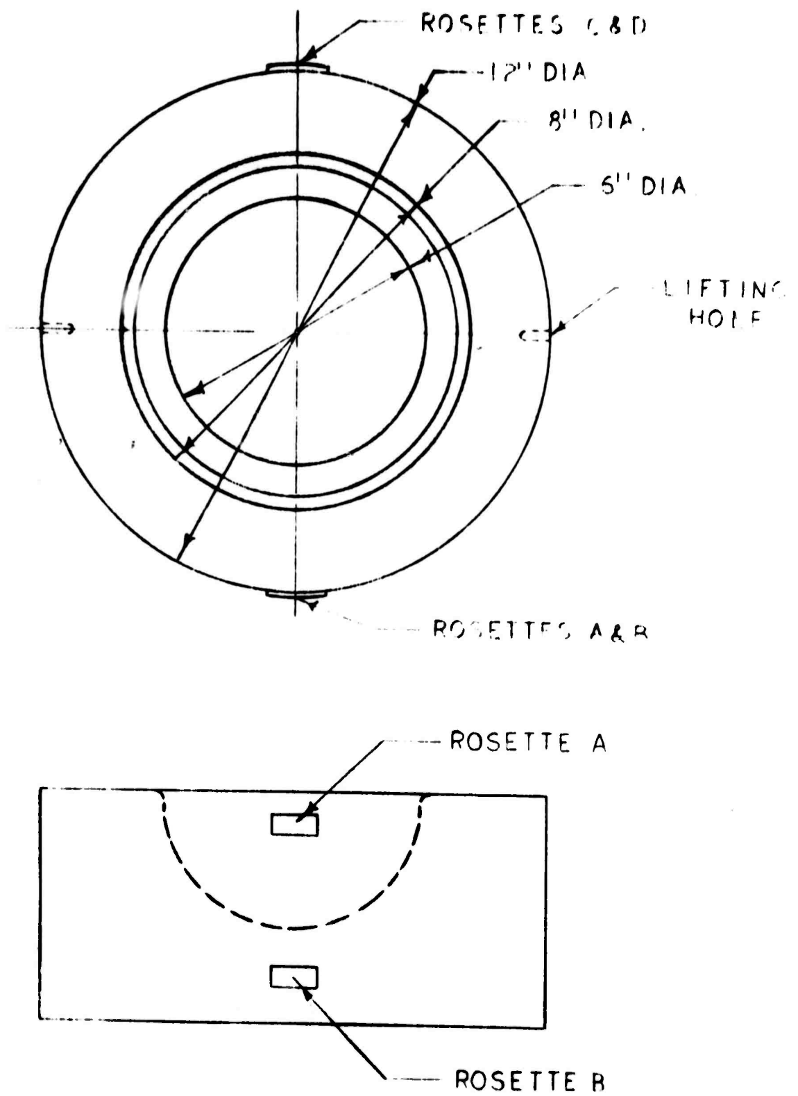
Figure 1 Die-Strain Gage Configuration
