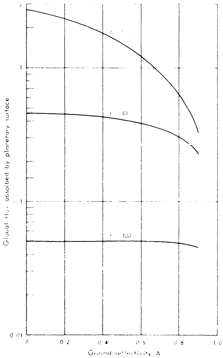
Fig. 3--Global Flux Absorbed versus Ground Reflectivity for Thickness \tau = 0.2, 10, \text{ and } 100 , normal incidence
