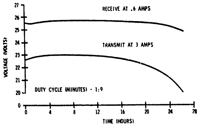
Figure 6. Transceiver Type Discharge at 125°F Ambient Temperature.
