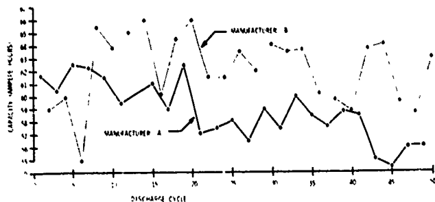
Figure 7. Capacity vs Recharge Cycles in Endurance Tests on Zinc-Air Battery BA-539 ( )/U.
