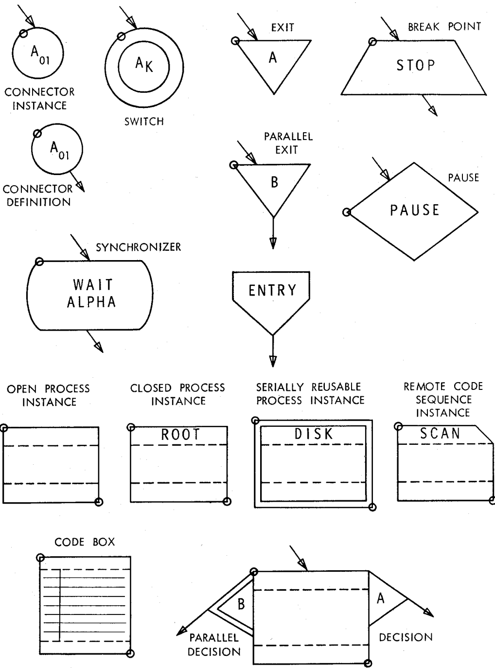
Fig. 3--Flowchart Symbols
