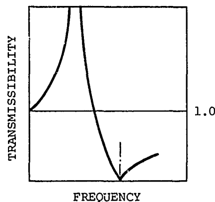
Figure 12 DAVI Vibration Isolation Curve
