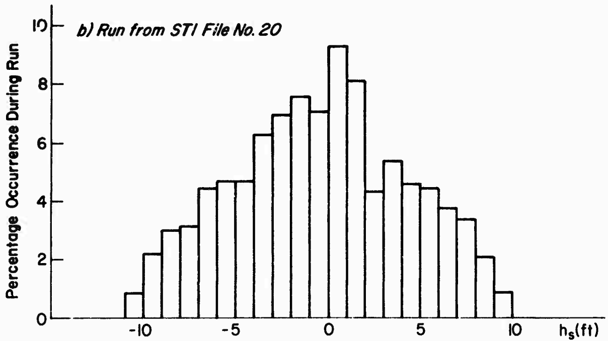
Figure C-3. Distribution of Amplitudes (From Mean) of Ship Heave ( h_s ) in Feet
