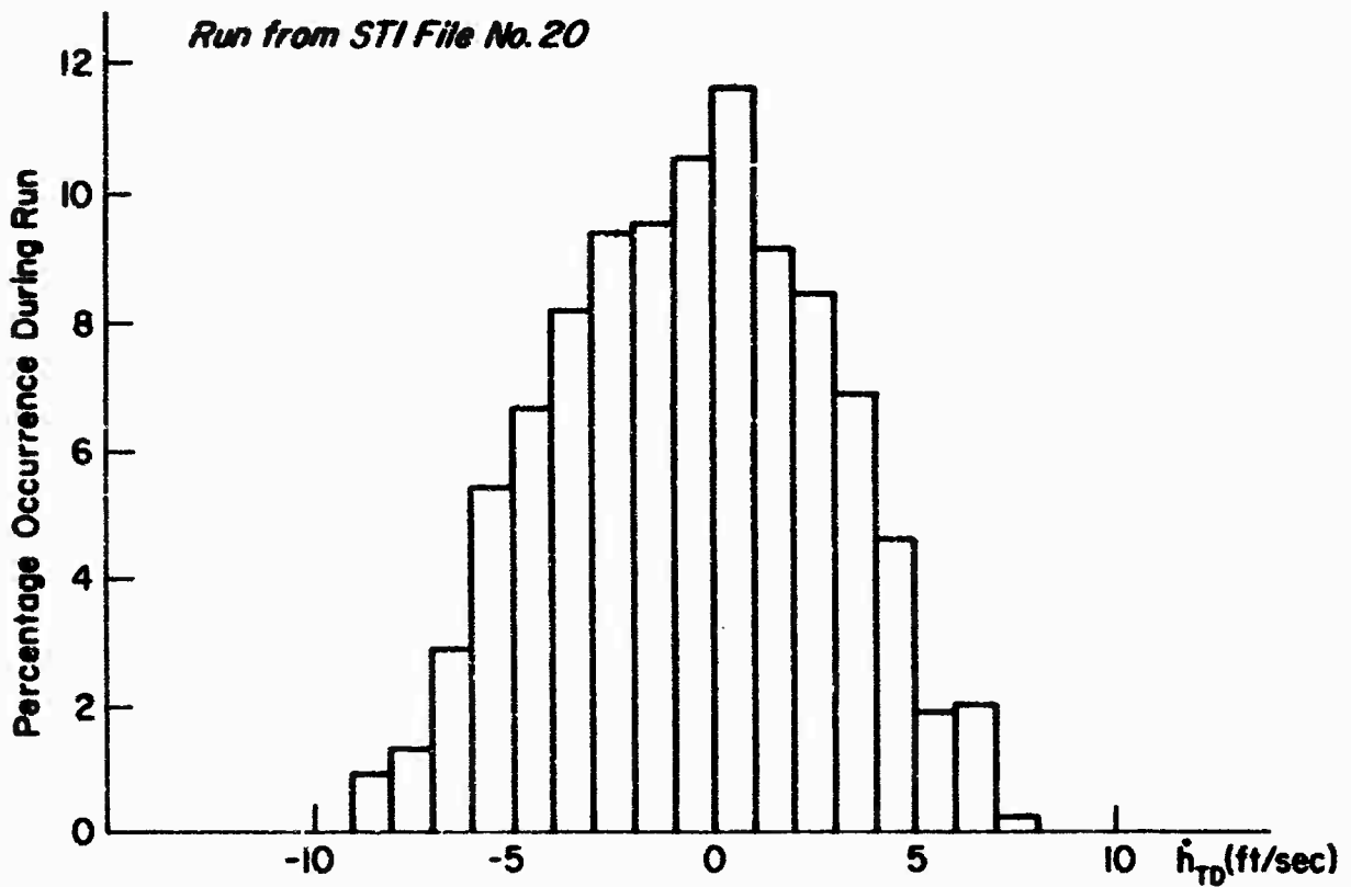
Figure C-7. Distribution of Amplitudes (From Mean) of Vertical Velocity of Touchdown Point ( \dot{h}_{TD} ) in Ft/Sec
