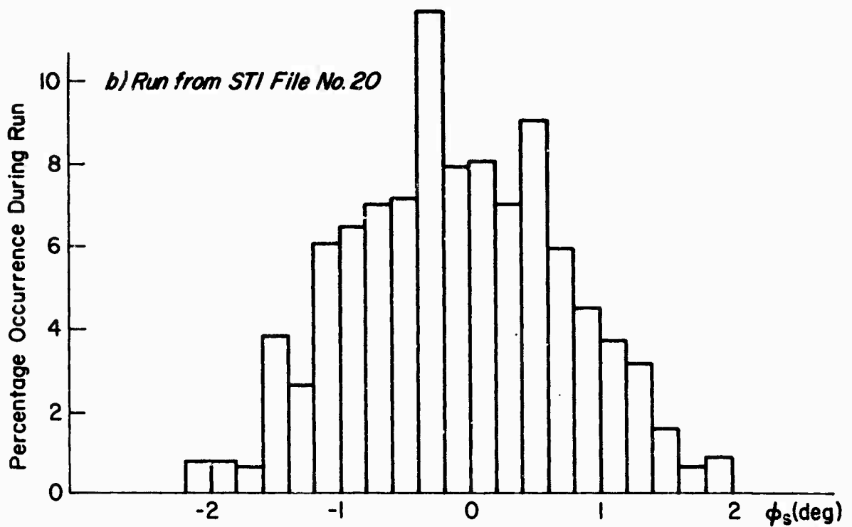
Figure C-2. Distribution of Amplitudes (From Mean) of Ship Roll Angle ( \phi_s ) in Degrees
