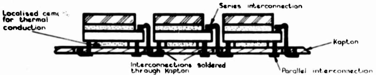
B Conventional contacts. Solder-through technique with localised mounting cement
