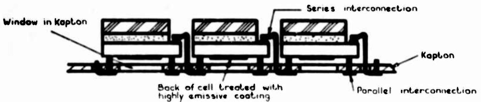
C Conventional contacts. Solder-through technique with windows in Kapton
