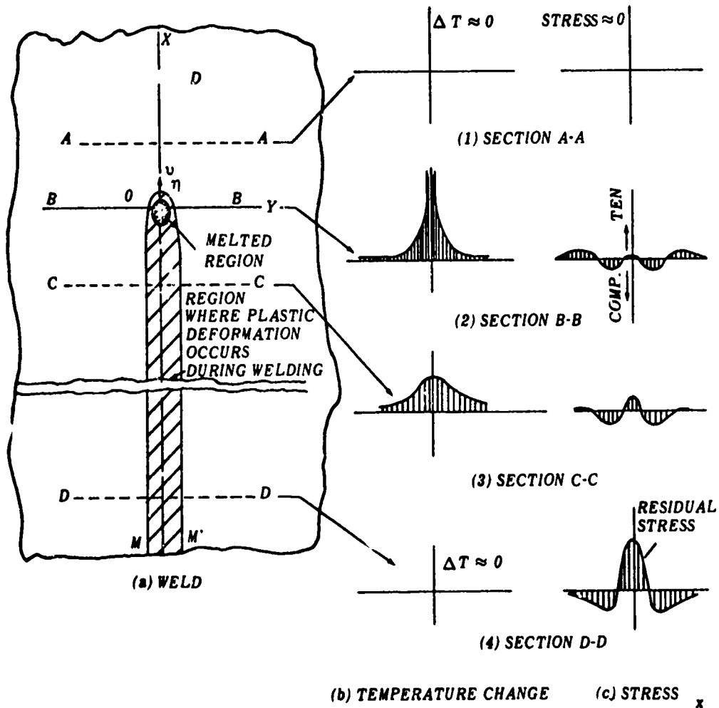
FIG. 1. Schematic Representation of Changes of Temperature and Stresses during Welding.
