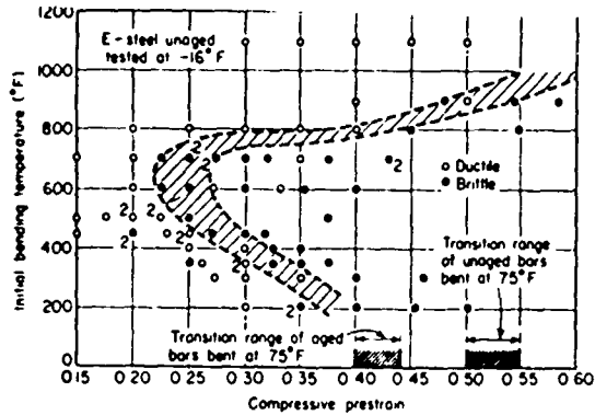
Fig. 10. Reversed-Bend Tests of Unaged Bars of E Steel Prestrained at Various Temperatures (64)
