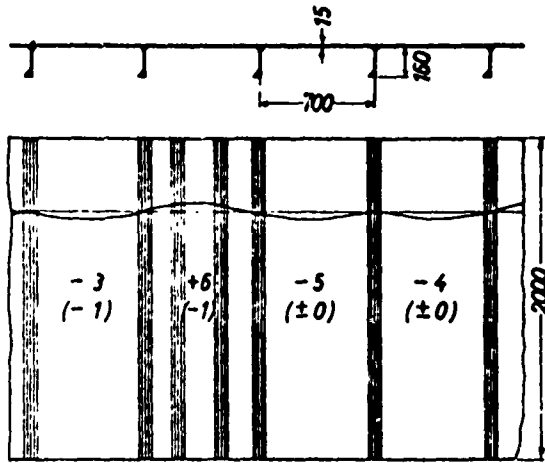
a. Straightening of a Hull Section
