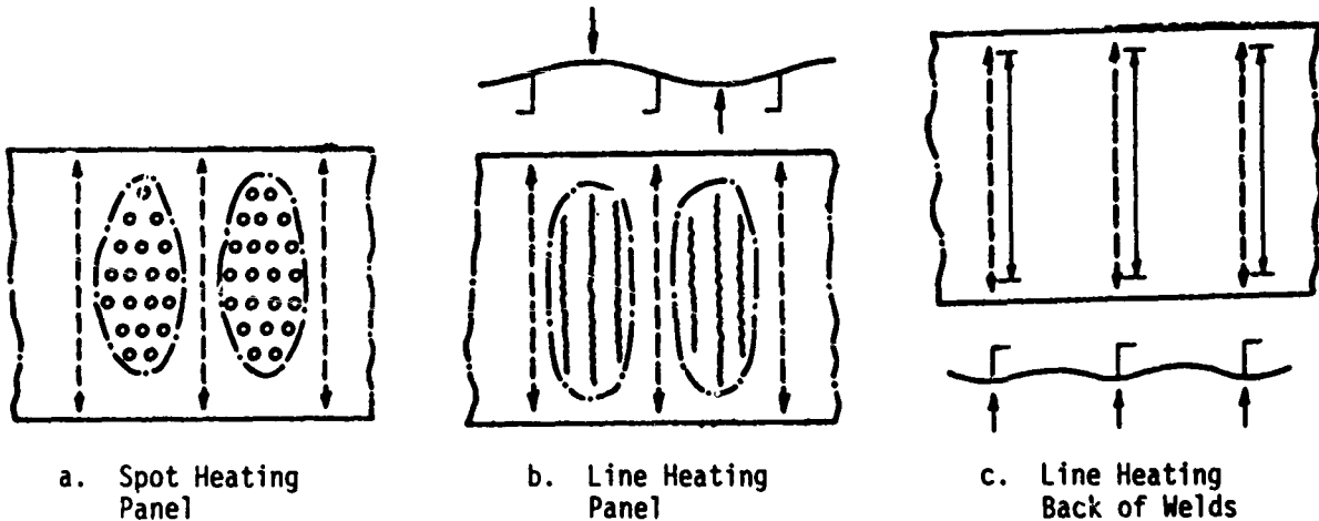
Fig. 6. Heating Patterns for Flame Straightening
