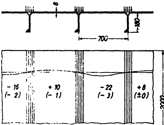
b. Straightening of a Deck Section
