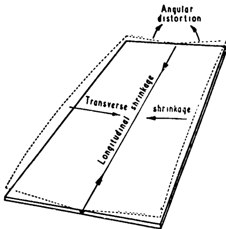
Fig. 2. Effects of Shrinkage, Causing Plates to Take Shape of Dotted Lines.
