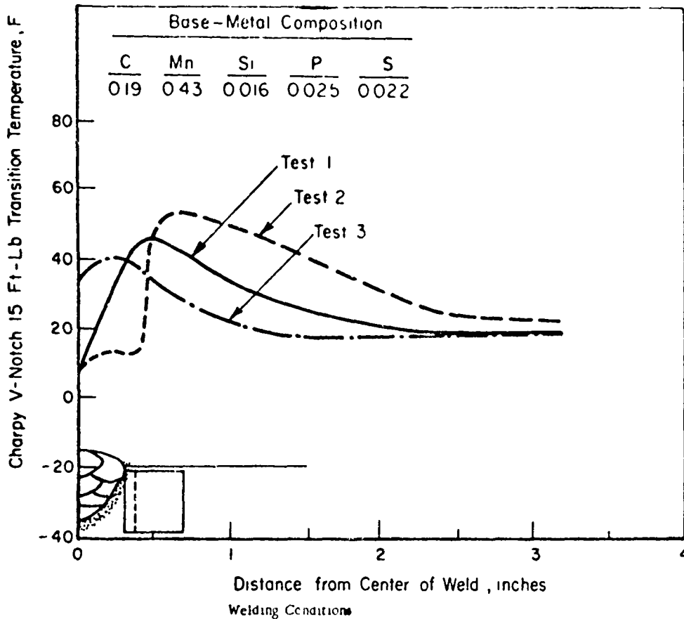
(a) For each pass. Fig. 12. Distribution of Charpy V-Notch 15-FT-LB Transition Temperature in Groove Welds in 1/2-inch-thick Mild-Steel Plates Made with Shielded Metal-Arc and Submerged-Arc Processes (68)
