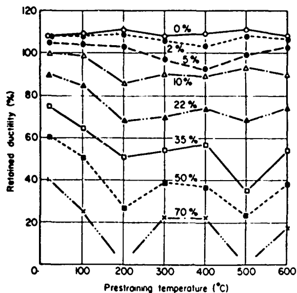
Fig. 8. Tensile Prestrain Tests for Cylindrical Specimens (61)
