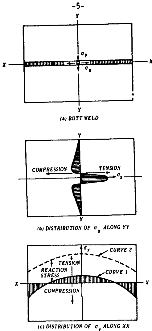
FIGURE 4. TYPICAL DISTRIBUTION OF RESIDUAL STRESSES IN BUTT WELD
