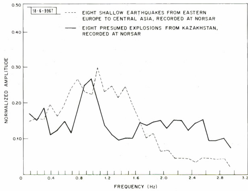
Fig. 1-1. Comparison of spectra of earthquakes and presumed explosions at NORSAR.
