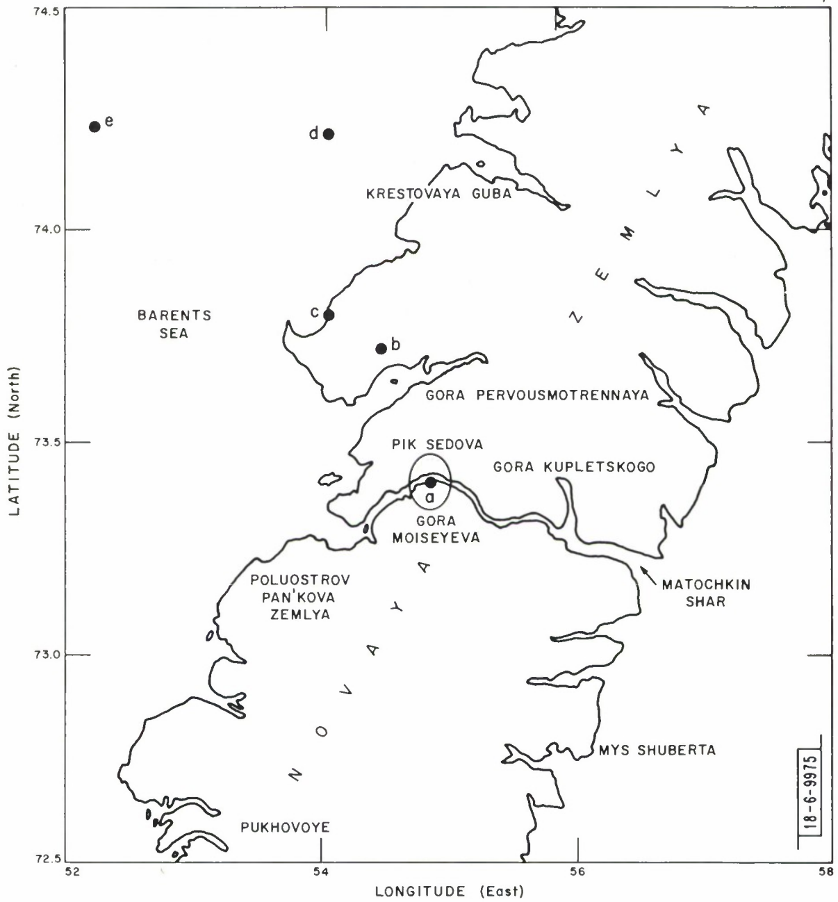
Fig. I-6. Migration of location of peak power for 27 October 1966, Novoya Zemlya event.
