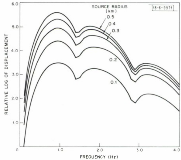
(d) Spectral effects of attenuation ( t^* = 0.6 ) and instrument response.
