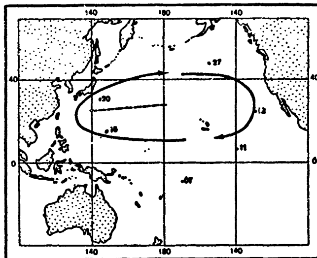
Fig. 1. Distribution of \text{Cs}^{137} in the surface waters of the Pacific Ocean, \mu\mu\text{c}/\text{l} [2].
