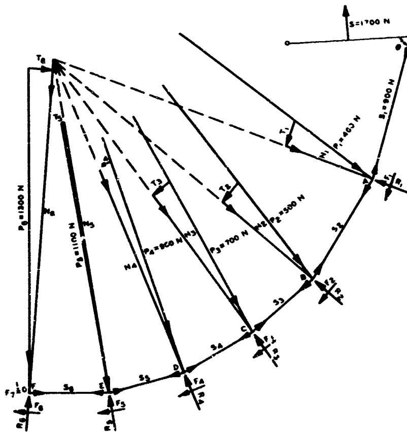
Fig. 14. Schema of the static system of the experimental wheel
