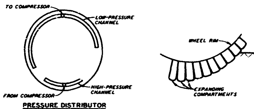
Fig. 28. Schema of a multicompartment tire
