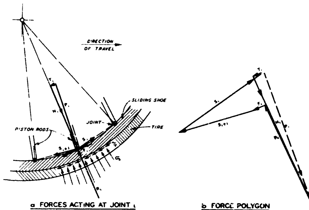
Fig. 13. Forces acting at articulated joint of experimental wheel normal stresses ( \sigma_s ) at the shoe-tire interface as shown in fig. 13. For simplicity, all forces are assumed to act directly at the joint. Because of the free articulation of these joints, the orientation of the tensile forces, S_i , is known to pass through the neighboring joints. Therefore, if the geometric conditions are known in the neighborhood of a given joint, the orientation of all forces acting on that joint are known. However, except for P_i , which is known from equation 9 and which can be decomposed into its normal and tangential components, N_i and T_i , the magnitudes of the four remaining forces are unknown and must be determined from the equilibrium conditions at the joint.
