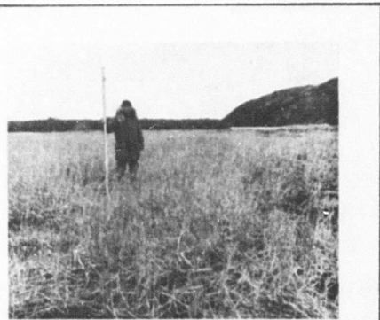
Fig. 32. Vegetated Flat.
