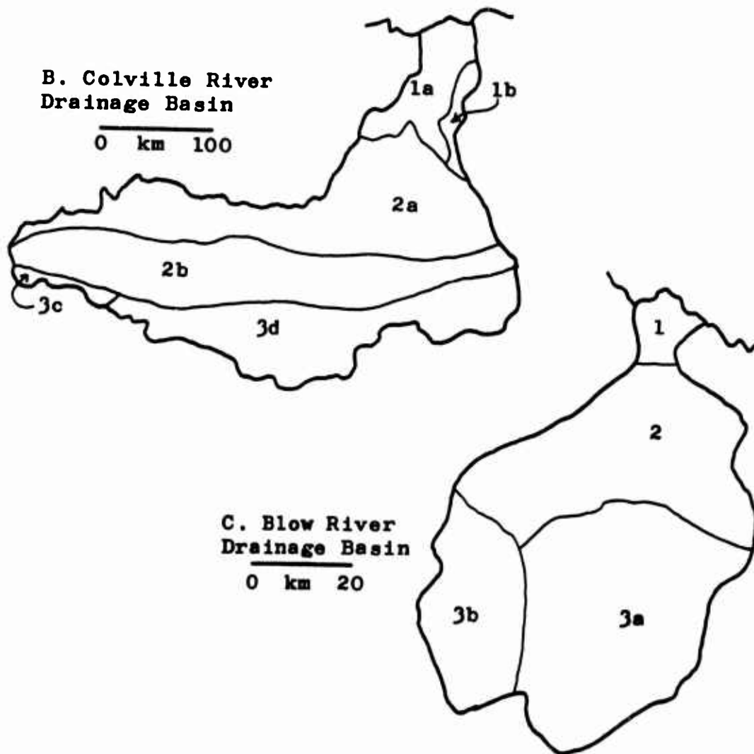
Fig. 3. Drainage Basins. See Table I for Divisions.
