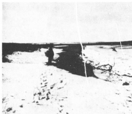
Fig. 66. Chute Cutoff Protected by Snow.
