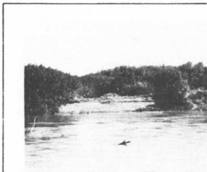
Fig. 29. Relict Channel Deposits, (B9-46).
