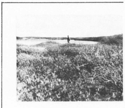
Fig. 33. Willow and Alder Vegetation on Mature Flat.
