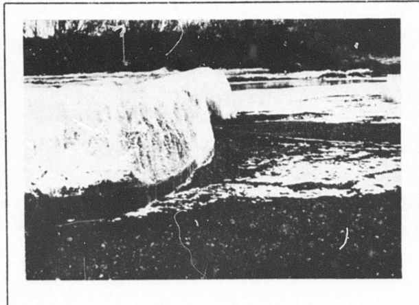
Fig. 57. Ice Shove on Gravel Bar (Blow).
