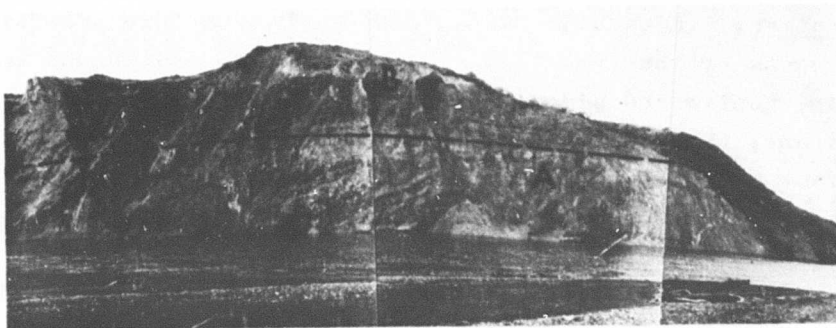
Fig. 6. Thirty-four Meter Bluff at Head of Blow River Delta.
