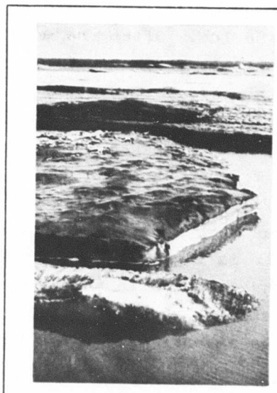
Fig. 70. Deposits on River Ice (Colville).
