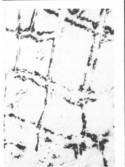
Fig. 16. Polygonal Surface Accentuated by Sediment Deposited during Sandstorm.
