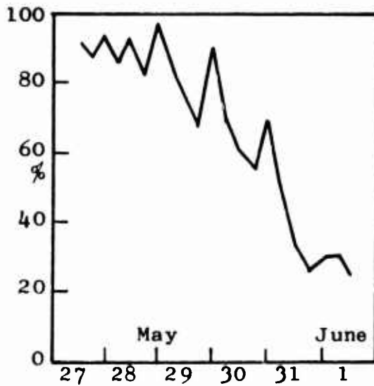
Fig. 13. Decay in Albedo, Barrow, 1964 (After Fig.4 in Ref. 23).
