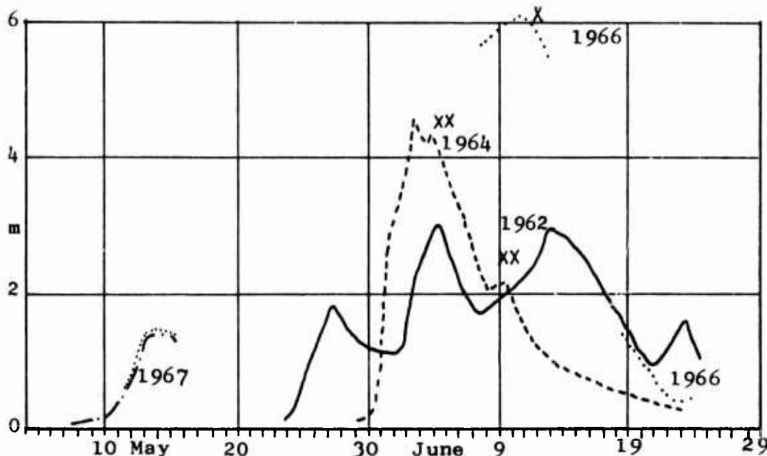
Fig. 18. Stage and Breakup, Selected Years, Colville Delta.
