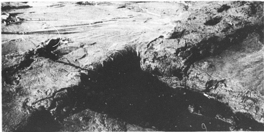
Fig. 17. Permafrost Table and Mud Flat Drainage.
