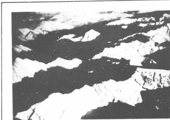
Fig. 4. Folded Sedimentary Rocks, Northern Brooks Range, Alaska.
