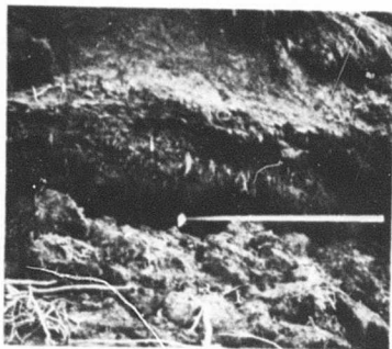
Fig. 76. Narrow Niche in Peat Bank (C1-22, Colville).
