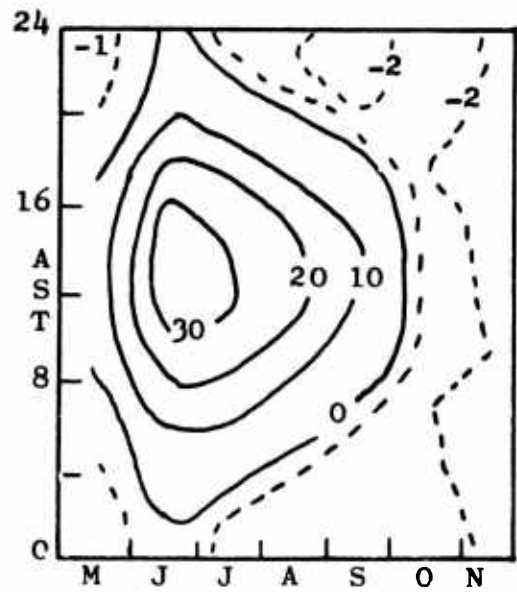
Fig. 14. Net Total Radiation, Barrow, 1964, mWcm^{-3} (After Fig.2 in Ref. 23).
