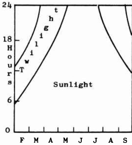
Fig. 10. Duration of Sunlight and Twilight at 70°N.
