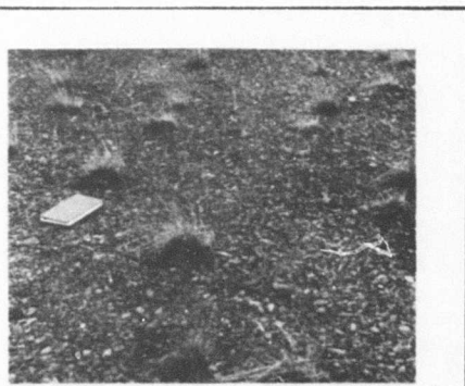
Fig. 30. Initial Colonization of Gravel Bar.
