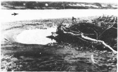
Fig. 80. Nonsymmetrical Scour Feature (Blow).
