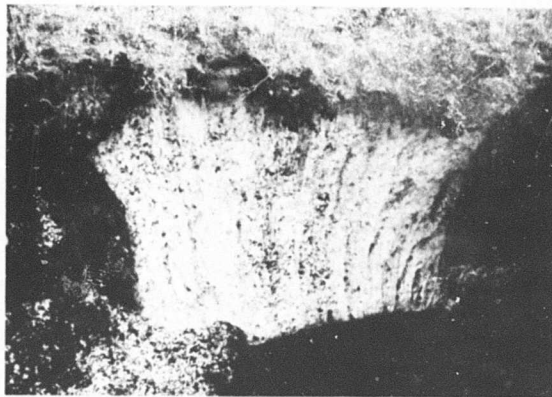
Fig. 49. Ice Wedge in Peat, 5 m wide.
