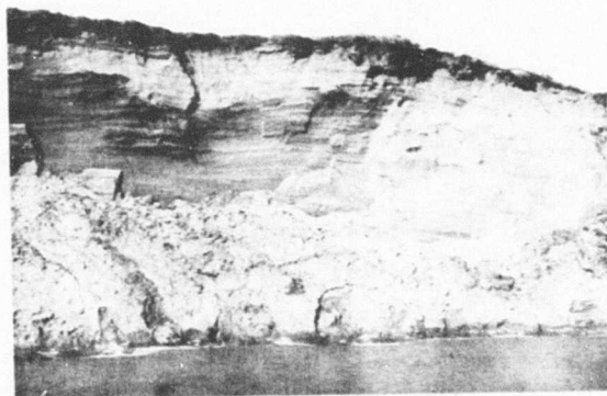
Fig. 42. Sand Dune Bank, Colville Delta (B7-32).
