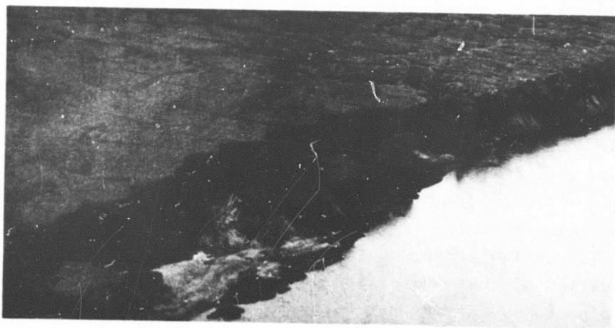
Fig. 75. Collapse of 8-m High Bank, 1962 (B7-32, Colville).
