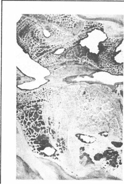
Fig. 47. Ice-Wedge Polygons
