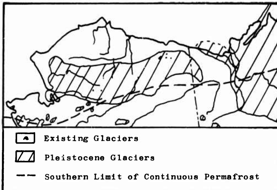
Fig.2. Glaciation and Permafrost (After 20 and 78).
