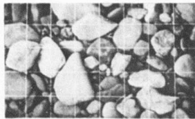
Fig.28. Representative Bar Materials. Scale, 5 cm per unit.
