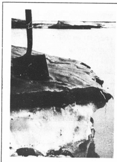
Fig. 69. River Deposits on Snow (Colville).
