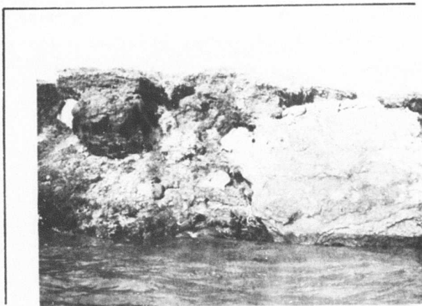
Fig. 41. Peat Bank, Colville Delta (B8-32).
