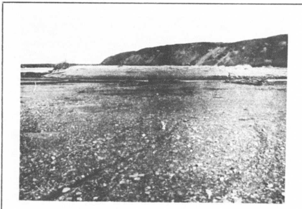
Fig. 61. Gravel Bar Scour Trails (Blow).
