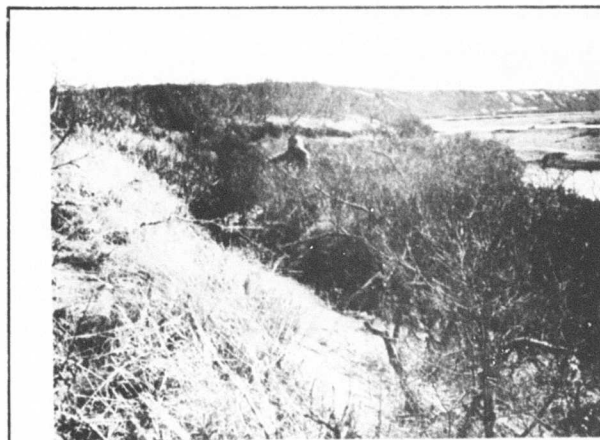
Fig. 9. Cutbank Vegetation.
