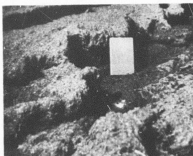
Fig. 36. Organic Beach, (E7-58).
