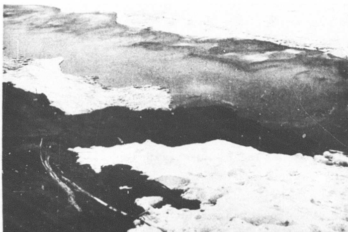
Fig. 64. Sand from Sand Dune Deposited on Snow and River Ice by Melt Water.
