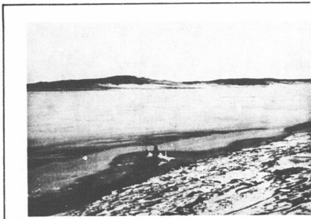
Fig. 21. Colville River Refrozen After Early Thaw, May 1967.
