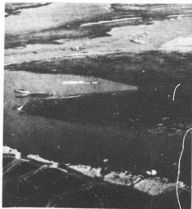
Fig. 72. Deposits on Lake Ice as Result of River Floods (D4-65, Colville).
