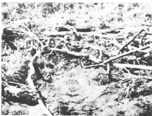
Fig. 59. Ice-Deposited Debris (Colville).
