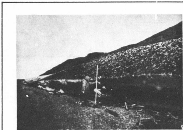
Fig. 23. Snowbank on Aug. 15, 1967 (Blow).
