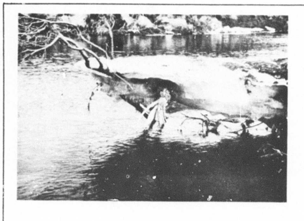
Fig. 60. Debris Incorporated in Ice Block (Blow).
