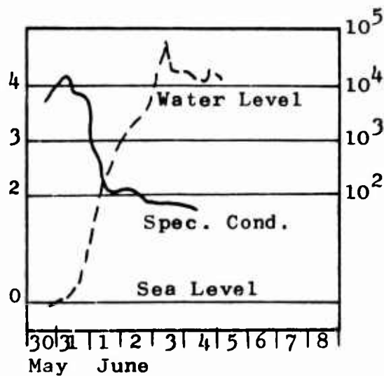
Fig. 19. Specific Conductance, Micromhos/cm 2 at 25° C. and Stage at Putu (C4-32), 1964.
