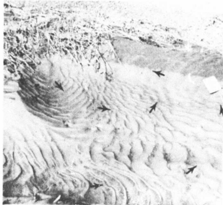
Fig. 81. Counter-Current Forms (B4-55, Blow).
