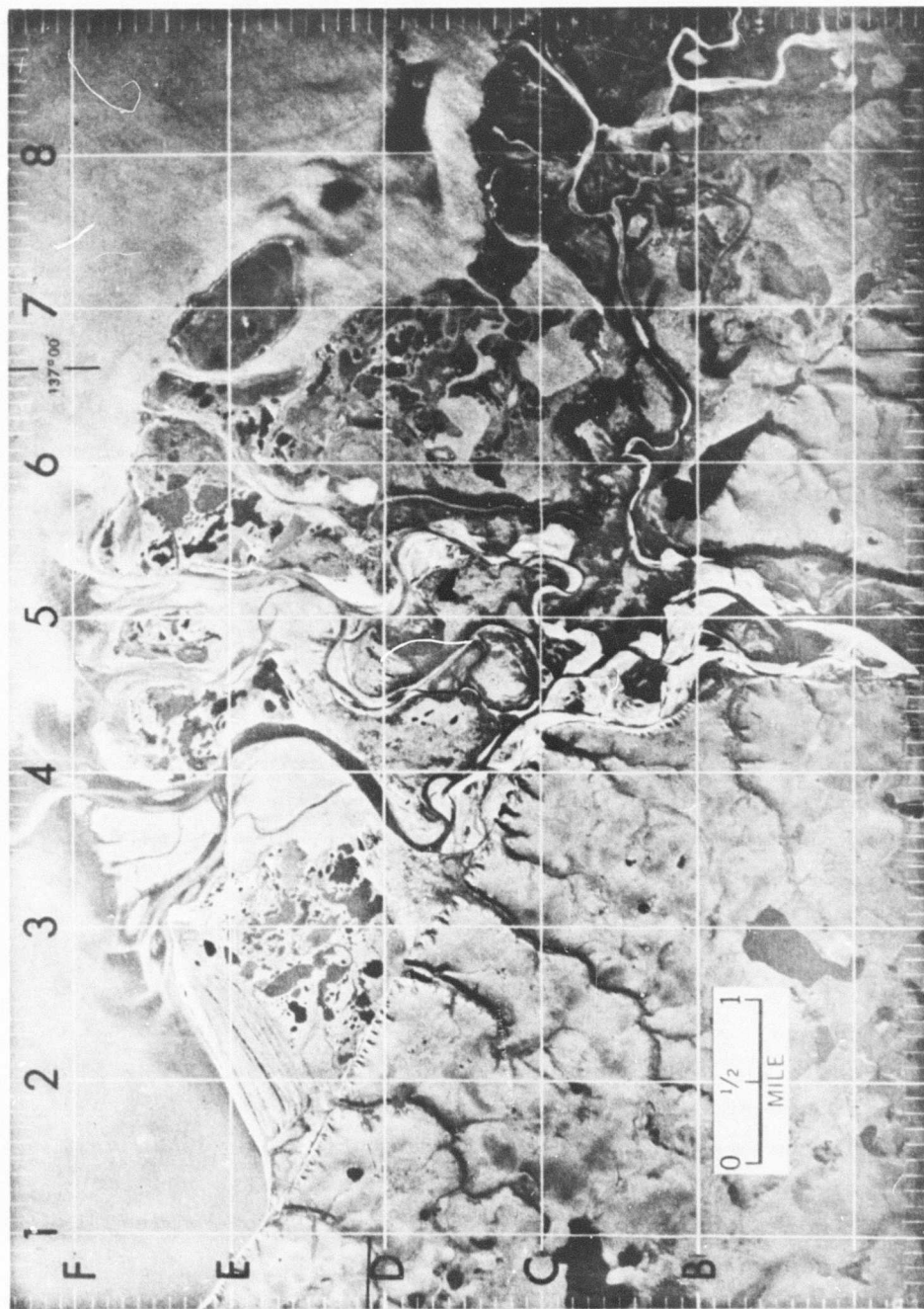
Fig. 24. Blow River Delta. Based on Photo No. 44, Flight Line A-13232, Air Photo Div., Eng. Mines & Res., Canada, 1957.
