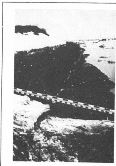
Fig. 68. Sediment Deposited on Snowbank (Colville).
