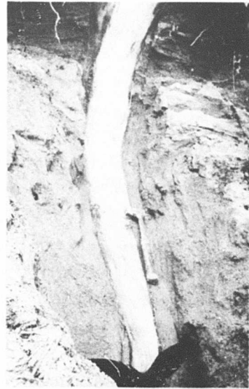
Fig. 48. Ice Wedge in Sand.
