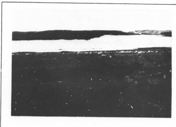
Fig. 63. Meltwater Erosion on Mud Flat (Colville).
