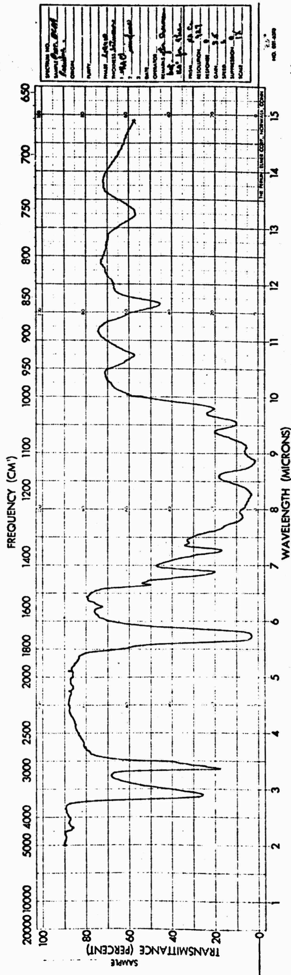
FIGURE 11 QUALITATIVE IR SPECTRA FOR DISTILLATION RESIDUE AFTER 4 HOURS AT 161°C
