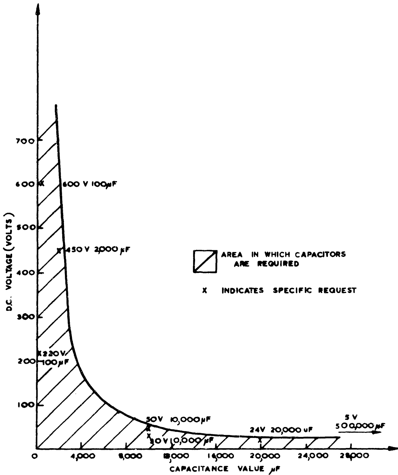
FIG. 5 GRAPH SHOWING VOLTAGE/CAPACITANCE REQUIREMENTS FOR FILTERS. (RIPPLE SUPPRESSION)
