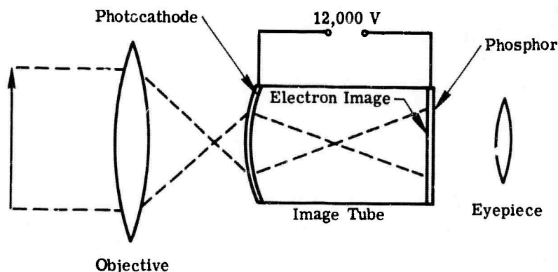
FIGURE 1. IMAGE-TUBE CONVERSION PROCESS
