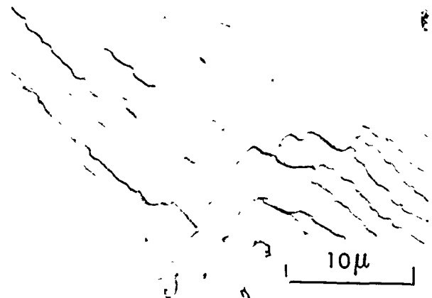
Figure 12. Stress-corrosion failure in Ti-13V-11 Cr-3Al in all- \beta condition failed in 0.6M KCl. 3500 X
