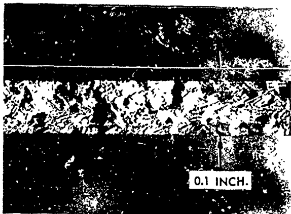
Figure 8. Optical fractograph of Ti-8Mn brittle failure in air (notched tensile specimen in \beta+\omega condition). 8 X
