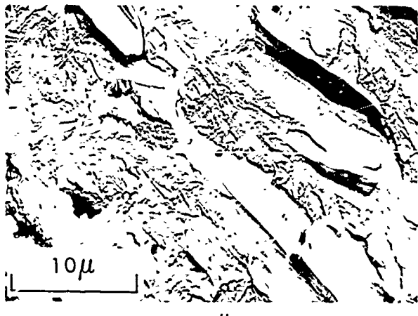
Figure 11. Alteration of fracture topography in Ti-8Al-1Mo-1V by variation of applied stress intensity (K). (a) low K; (b) high K 3500 X
