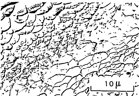
Figure 2. Correlation of dimple size and ductility in Ti-11.6Mo. Ductility decreases from: (a) all- \beta condition (70% elong.) to (b) \alpha + \beta condition (14% elong.) to (c) \beta + \omega condition (0% elong.). 3500 X
