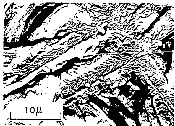
Figure 13. Stress-corrosion failure in Ti-6Al-4V illustrating cleavage in the \alpha phase and ductile fracture in the \beta phase, failed in 0.6M NaCl. 3500 X
