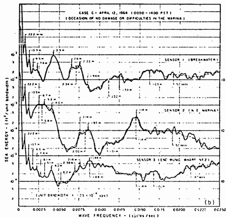
FIGURE 26 SEA-ENERGY SPECTRA FOR MA SENSOR LOCATIONS IN MONTEREY HARBOR: (a) FEB. 11, 1964 (CASE A); (b) APRIL 12, 1964 (CASE C)
