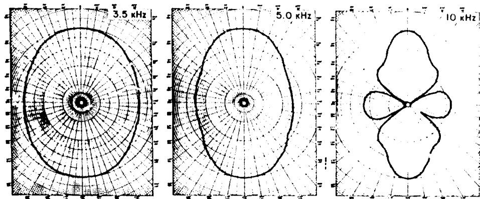
Fig. 4. Directivity patterns in the XY plane, type F43 transducer; shaded array.
