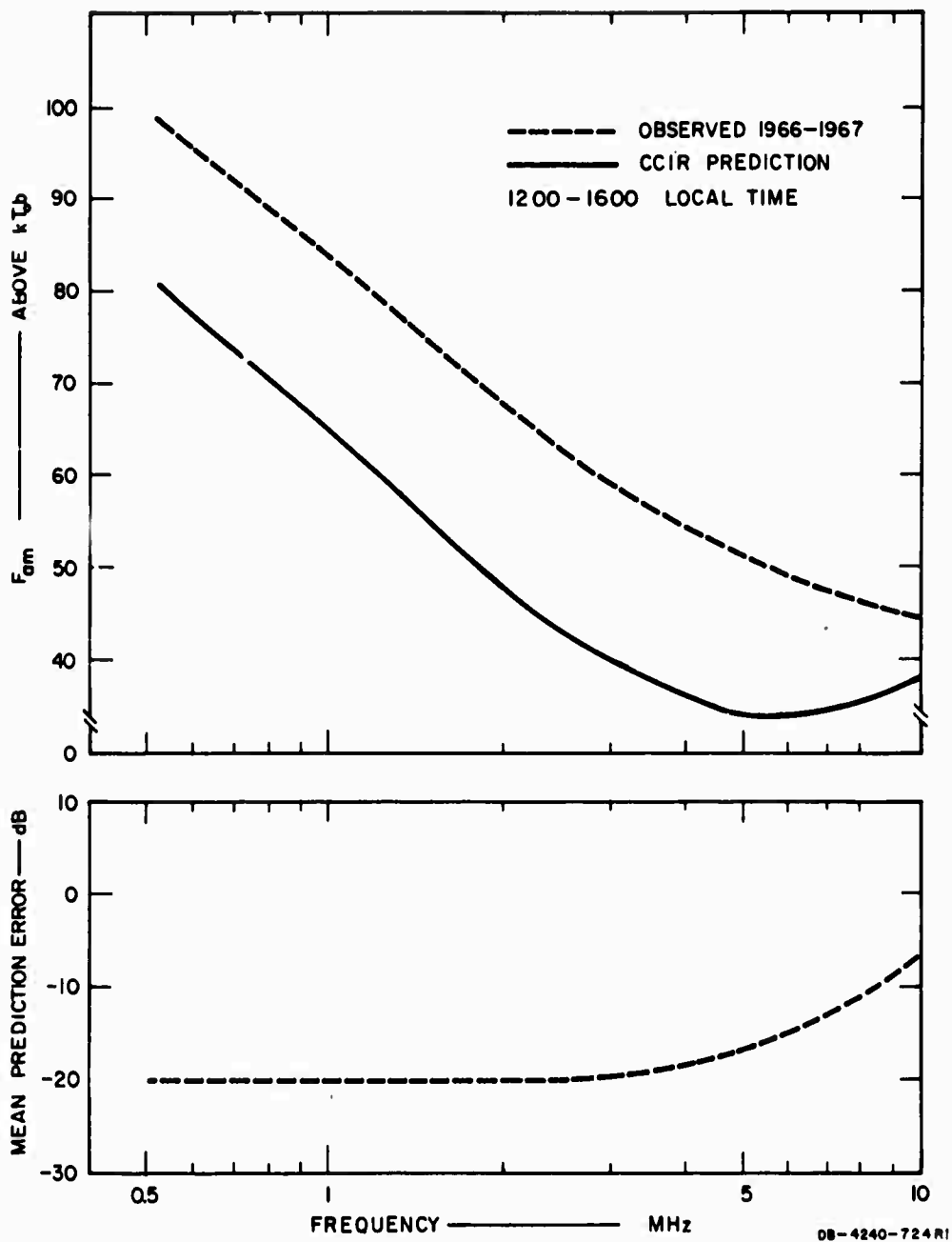
FIG. 36 COMPARISON OF OBSERVED AND CCIR-PREDICTED NOISE POWER, F_{am} , FOR A DAYTIME BLOCK (1200-1600)
