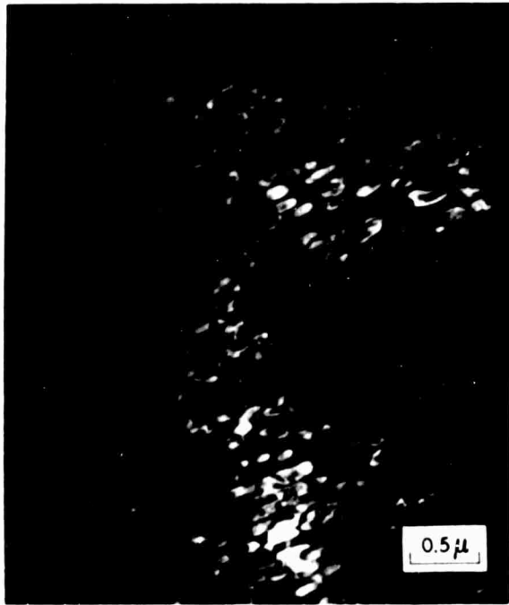
Fig. A-21 - Dark-field electron micrograph of omega formed during aging at 700° F for 500 hr.
