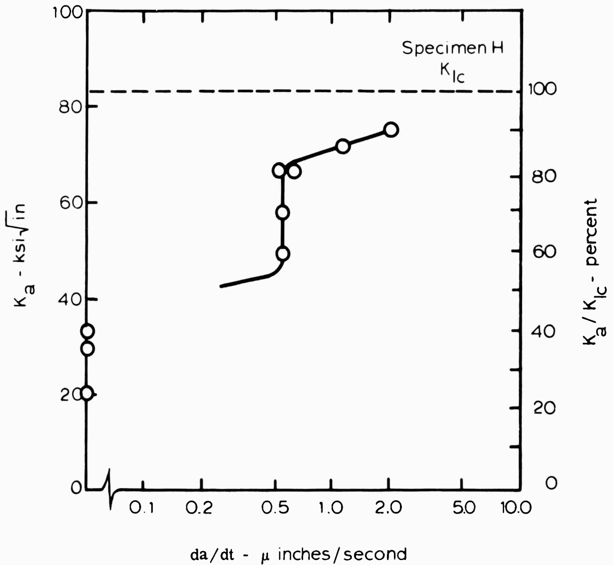
Fig. B-1 - Crack Growth Rate, da/dt , versus Applied Stress Intensity Factor K_a , and Ratio of K_a to K_{Ic} for 18Ni(250) Maraging Steel; Fully Heat Treated. Specimen Immersed in a 3-1/2% NaCl Solution at Room Temperature. Specimen with 25 percent Total Face Grooves (1/8 inch Cylindrical Grooves).
