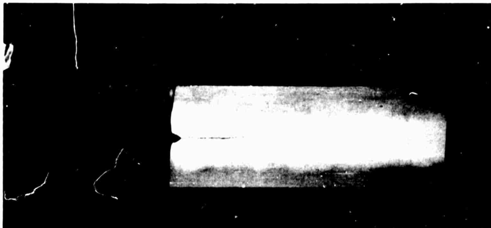
Fig. C-1 - Self-stressed uniform double-cantilever beam specimen with stress-corrosion crack. Dark region at left is paraffin used to insulate the loading screw from the crack area.
