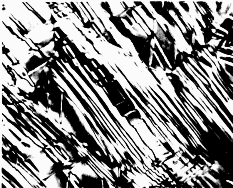
Fig. A-15 - Twins formed during 15% uniform elongation; Normarski interference contrast. \times 750
