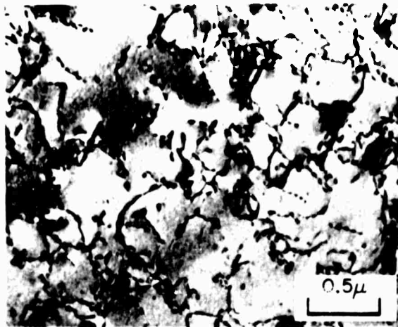
Fig. A3 - Dislocation arrangements in (a) Ti-70 (0.38 wt % oxygen) and (b) Ti-50A (0.12 wt % oxygen) after 3% to 4% deformation by rolling ( [0001]_{\alpha} zone axes).
