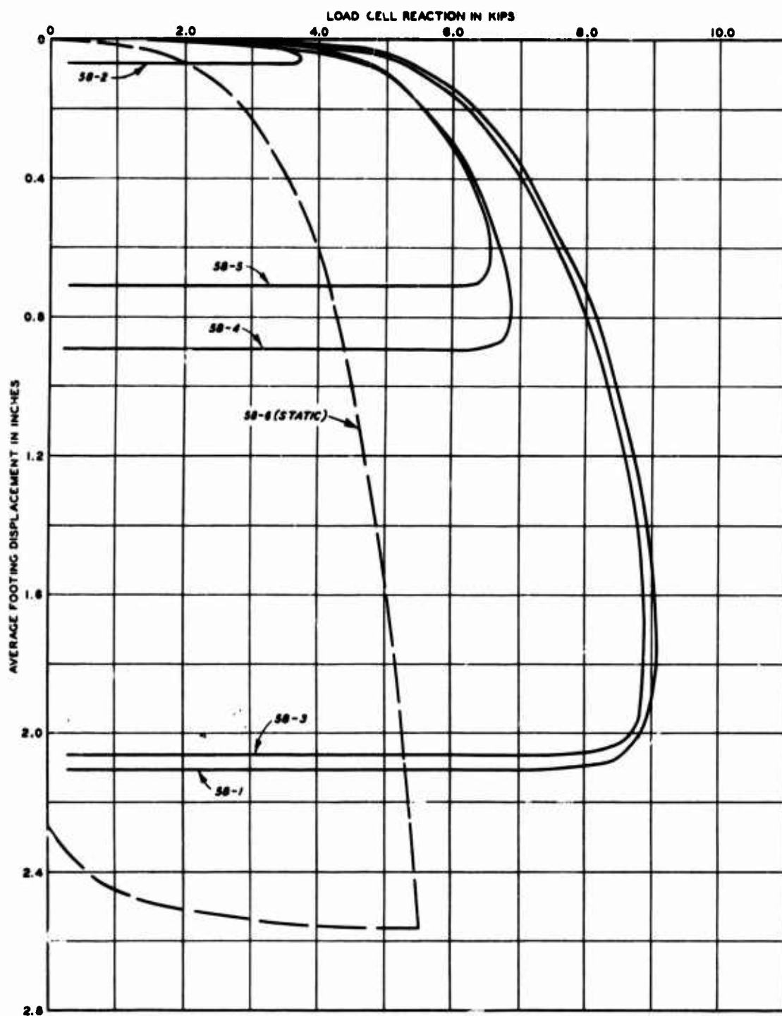
Figure D.11 Load-displacement curves, cart 58.
