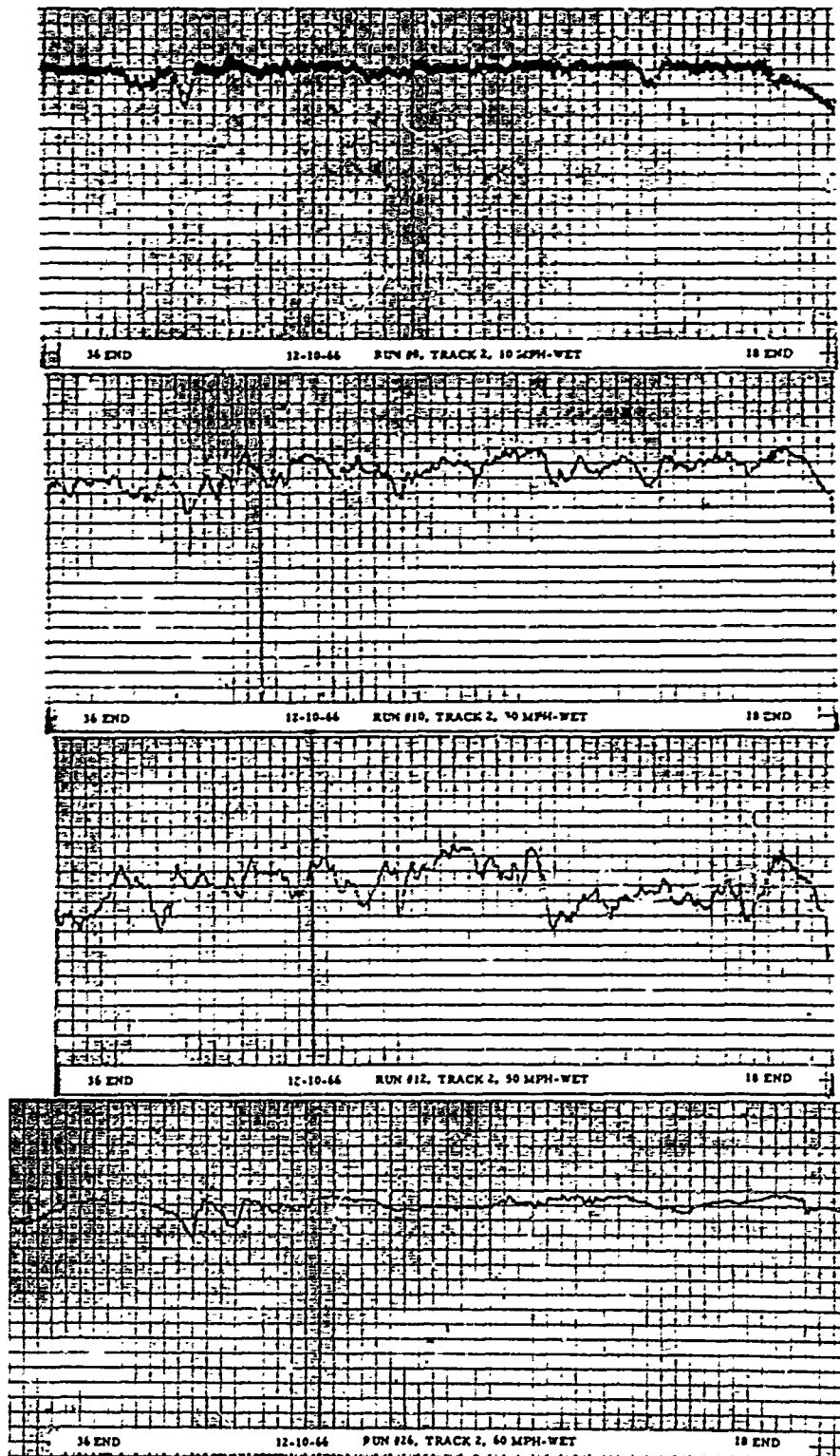
BEFORE GROOVING - TRACK 2, EAST RUNWAY EDGE WET TESTS
