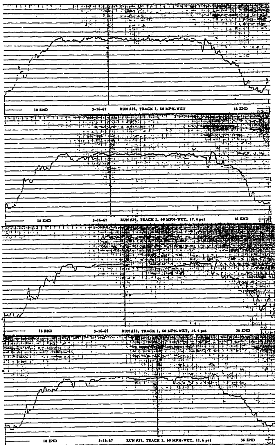
BEFORE GROOVING - TRACK 1, CENTERLINE WET TESTS
