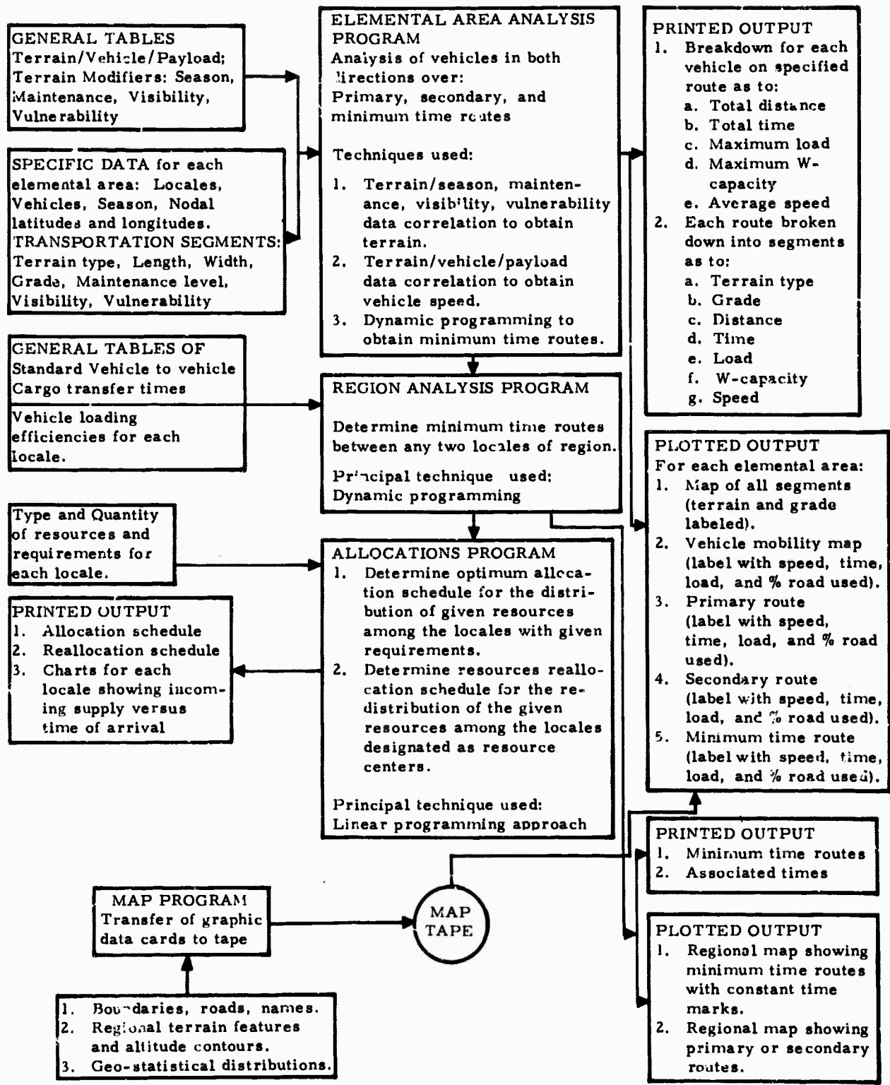
Figure 1. SIMDATS Functional Flow Diagram
