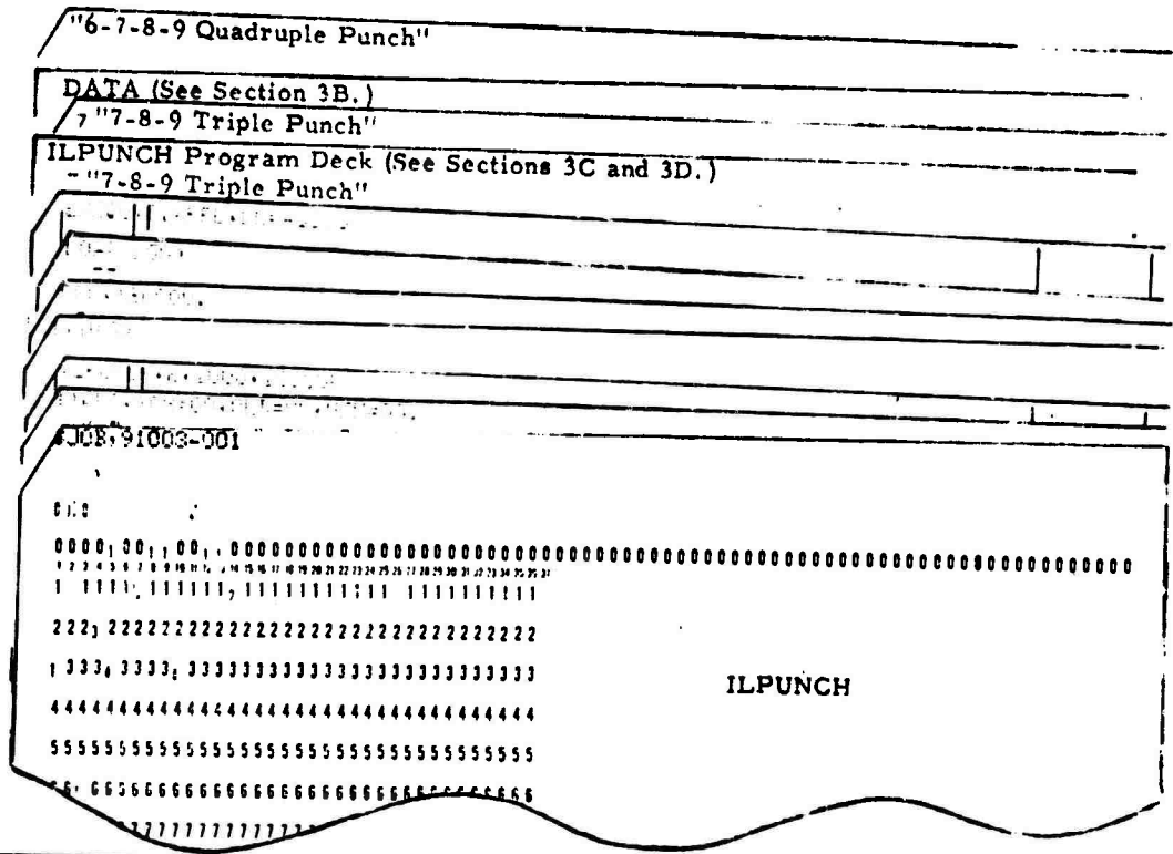
Figure 2. ILPUNCH Deck Setup
