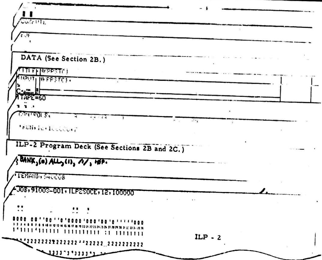
Figure 1. ILP-2 Deck Setup
