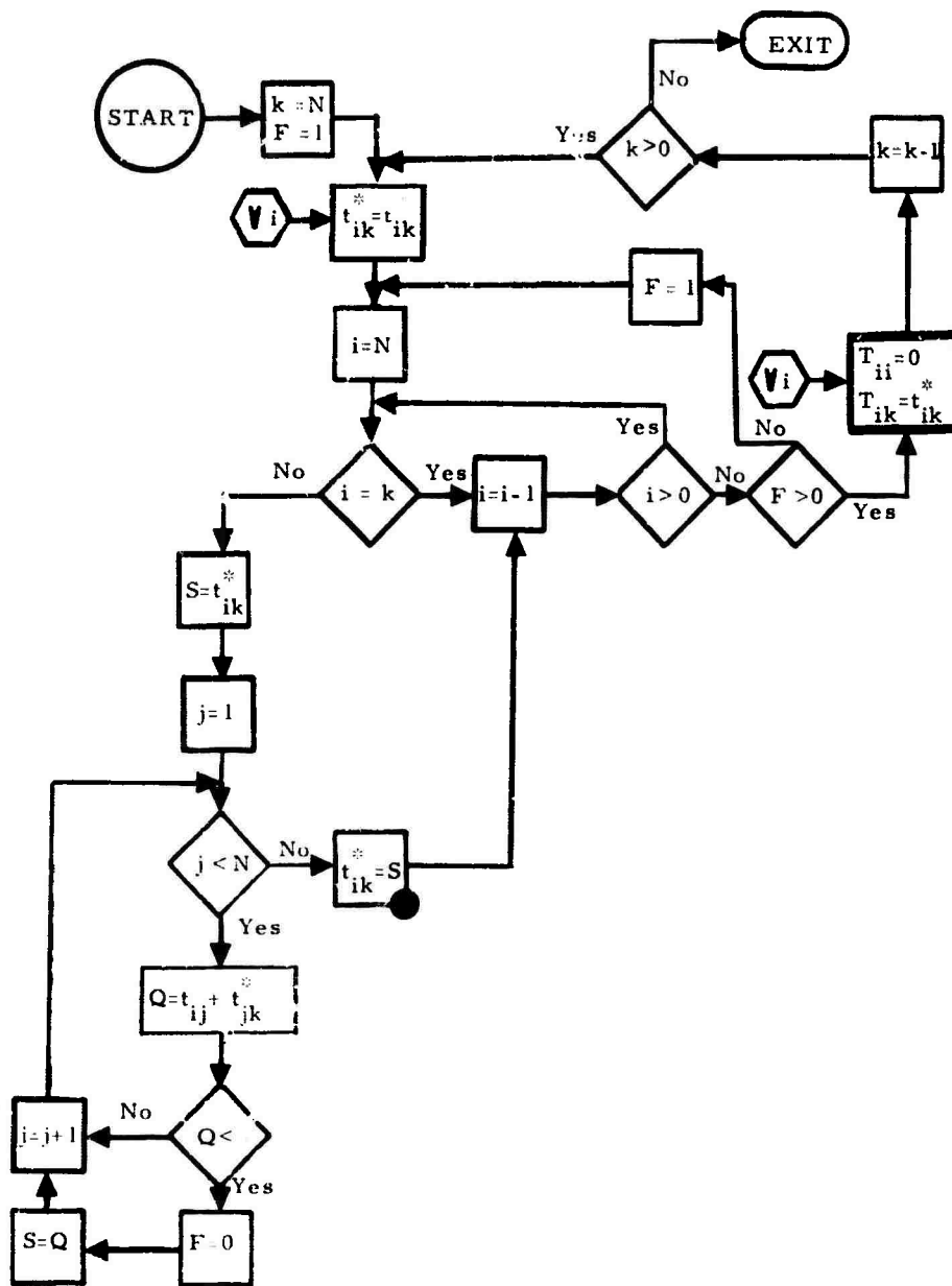
Figure 3. Simplified Program Logic
