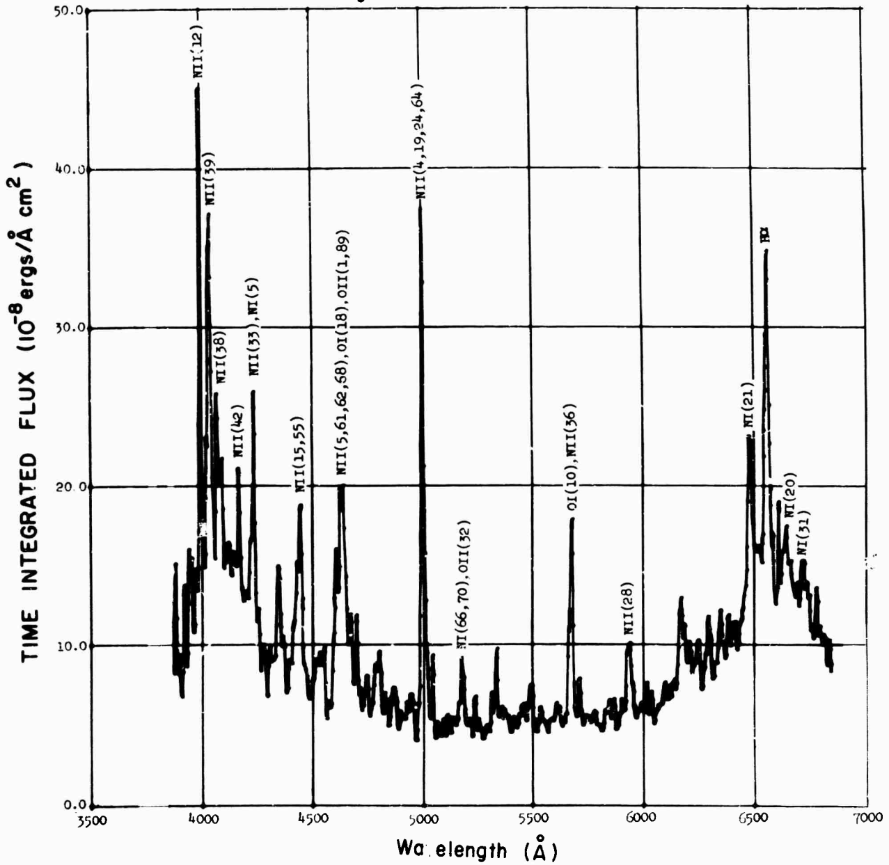
Fig. 17. Flux at spectrograph entrance pupil from ~17-meter length of channel, uncorrected for rain transmission. Subsequent return stroke.
