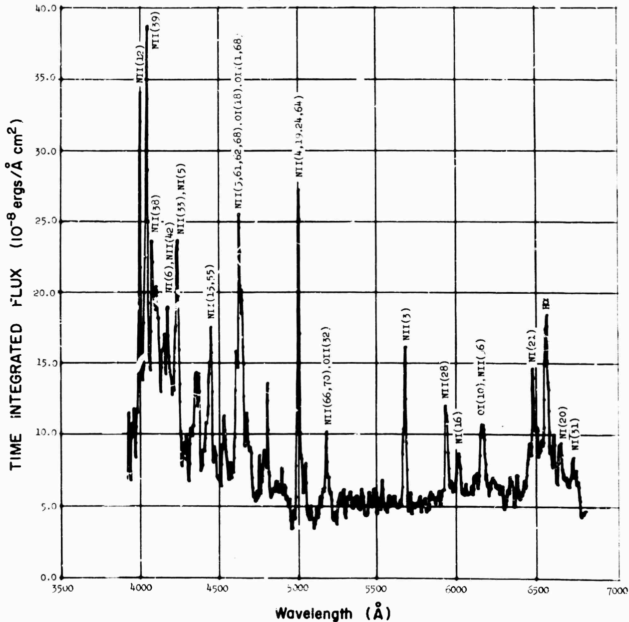
Fig. 24. Flux at spectrograph entrance pupil from ~21-meter length of channel, uncorrected for rain transmission. First return stroke.
