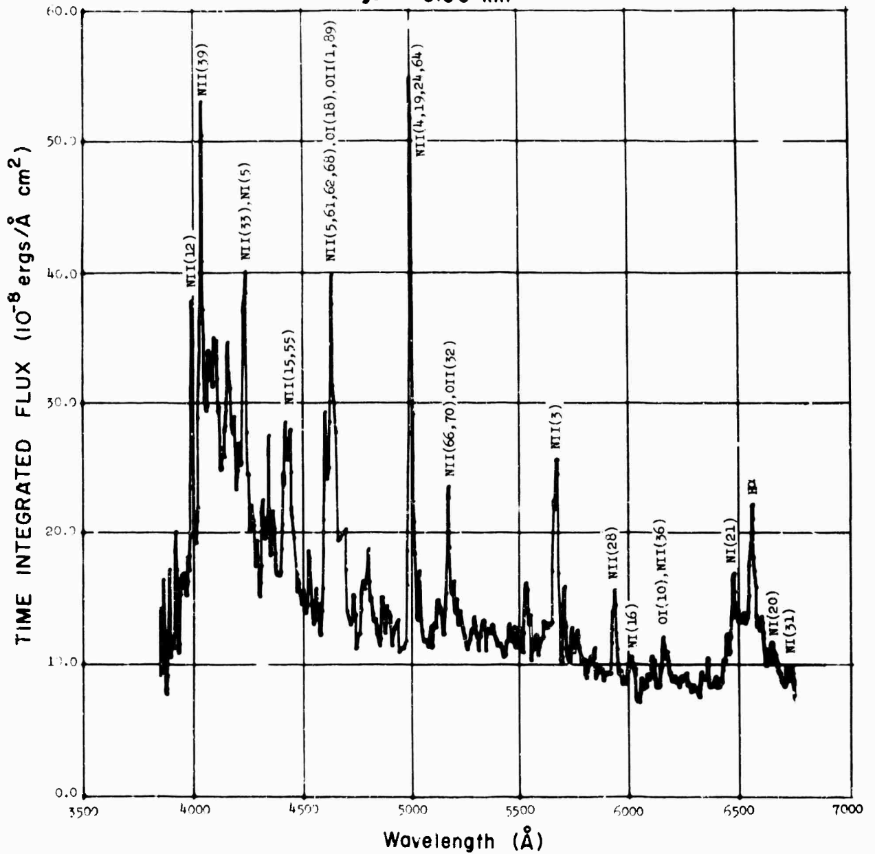
Fig. 20. Flux at spectrograph entrance pupil from ~16-meter length of channel, uncorrected for rain transmission. First return stroke.
