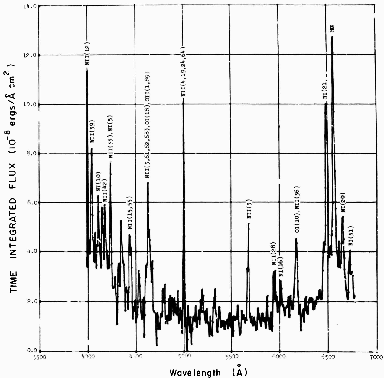
Fig. 12. Flux at spectrograph entrance pupil from ~16-meter length of channel, uncorrected for rain transmission. Subsequent return stroke.
