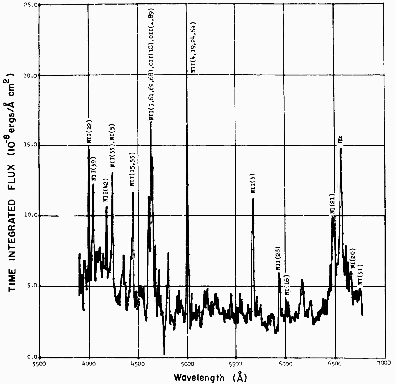
Fig. 18. Flux at spectrograph entrance pupil from ~ 16-meter length of channel, uncorrected for rain transmission, First return stroke.
