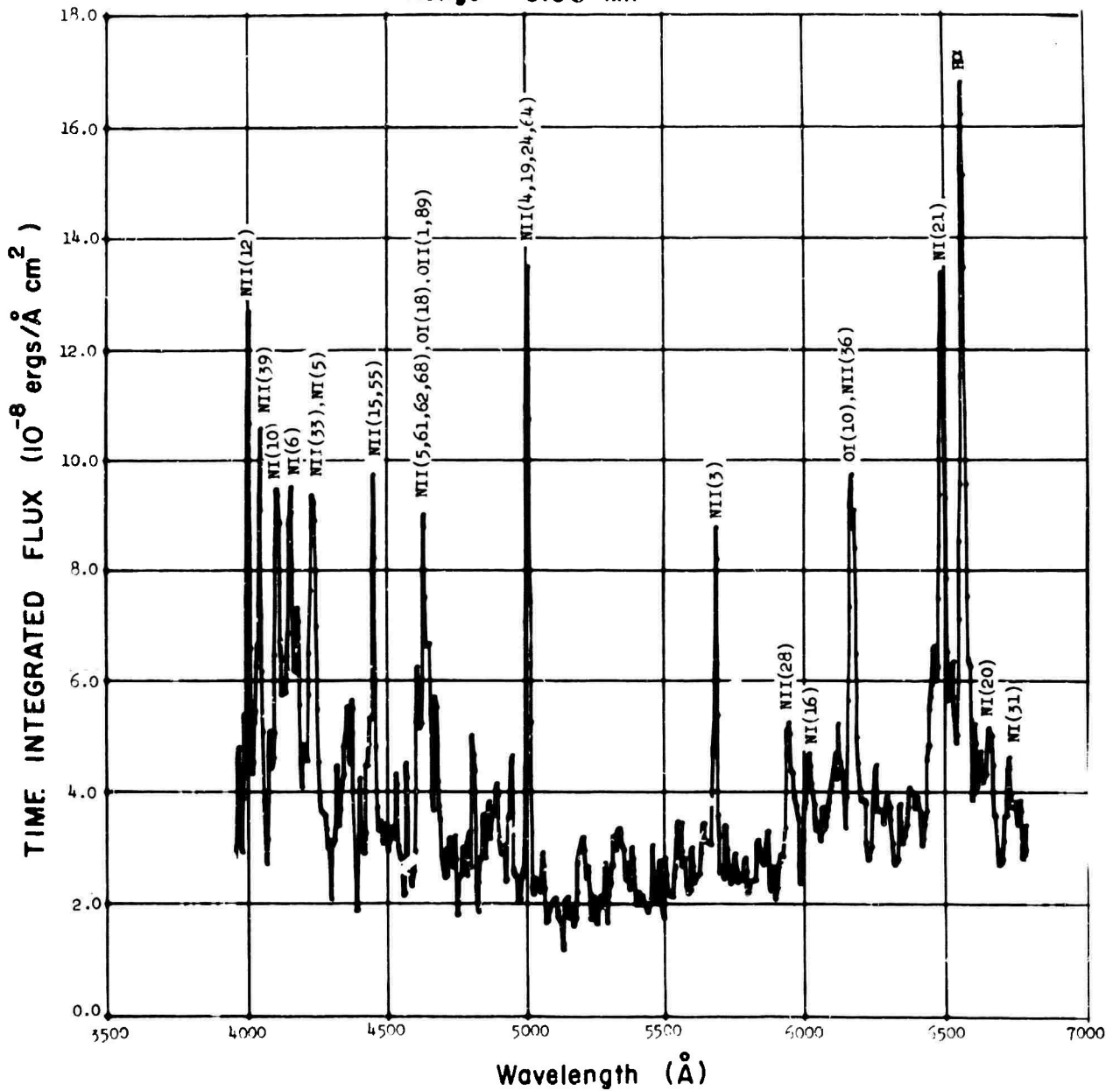
Fig. 14. Flux at spectrograph entrance pupil from ~16-meter length of channel, uncorrected for rain transmission. Subsequent return stroke.
