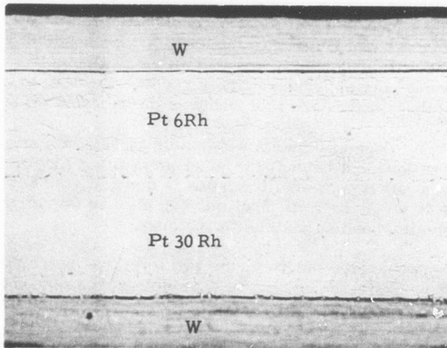
Microstructure
