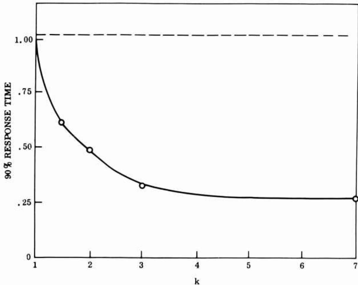
Figure 4. Multijunction Response Time as a Function of k , Where k = \tau_3/\tau_1 .
