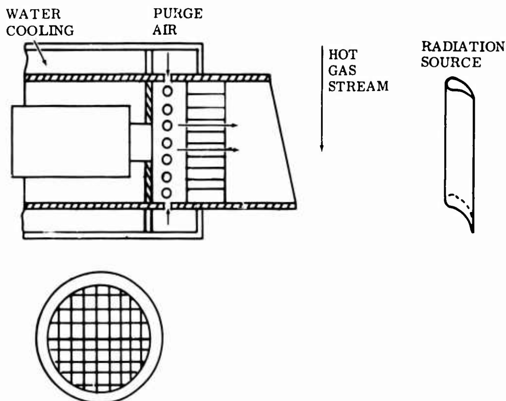
Figure 66. Air-Collimator Lens.
