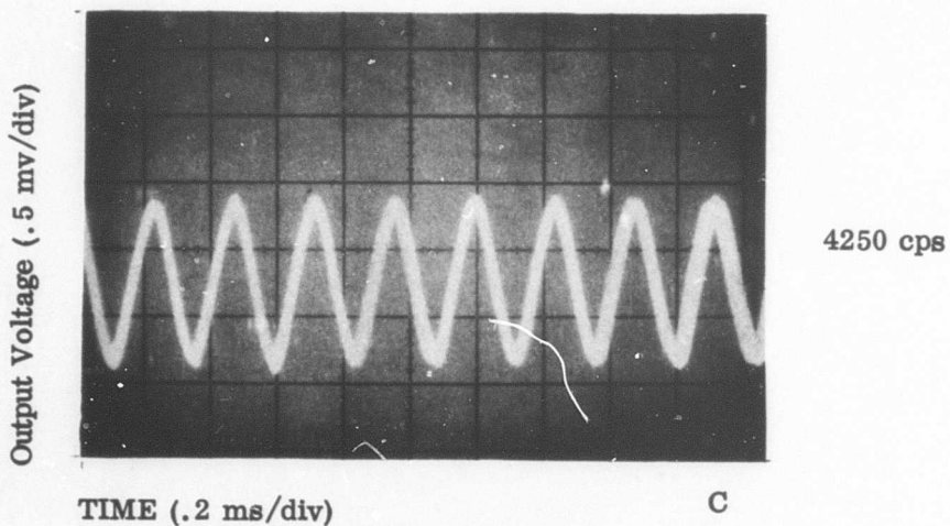
Figure 53. Output of Silicon Chip Pyrometer due to an Oscillating Target Temperature.
