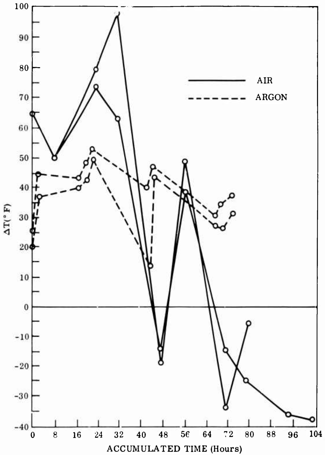
Figure 14. Drift Tests for Ir Versus Ir40%Rh Thermocouples.
