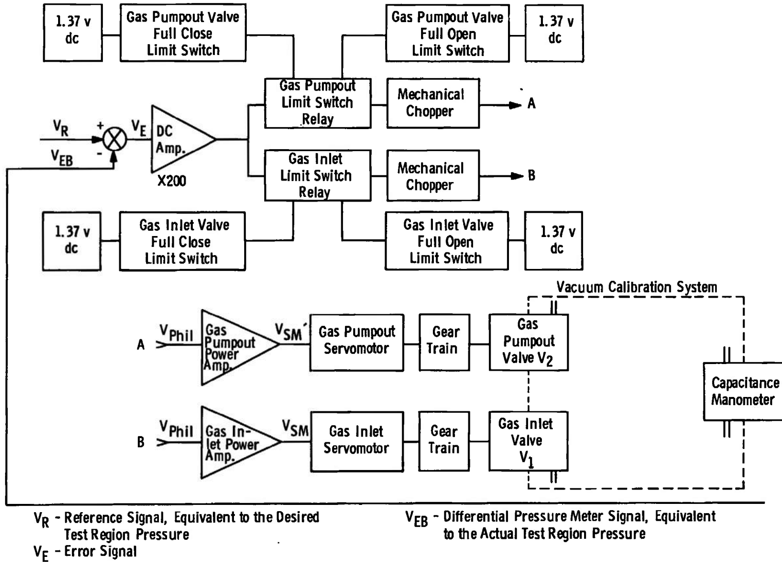
Fig. 6 Servocontrolled Gas Inbleed System Flaw Diagram
