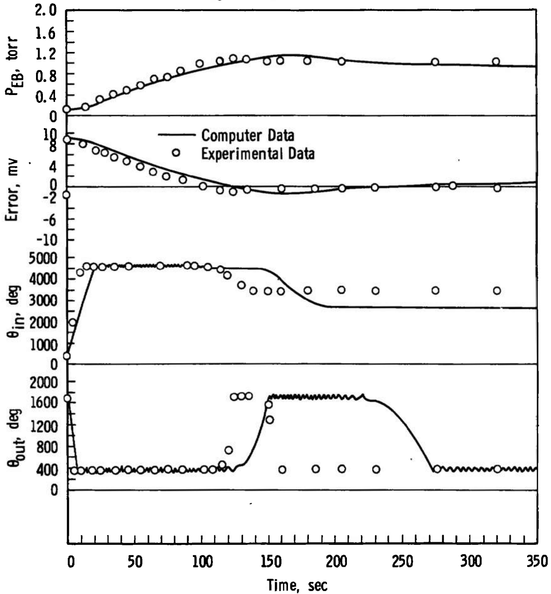
Fig. 16 Transient Response for a Forepressure Set Equal to 1.0 torr
