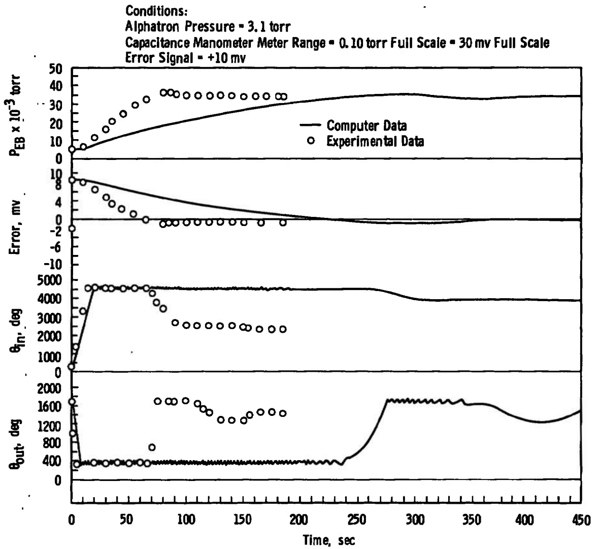
Fig. 13 Transient Response for a Forepressure Set Equal to 3.33 \times 10^{-2} torr
