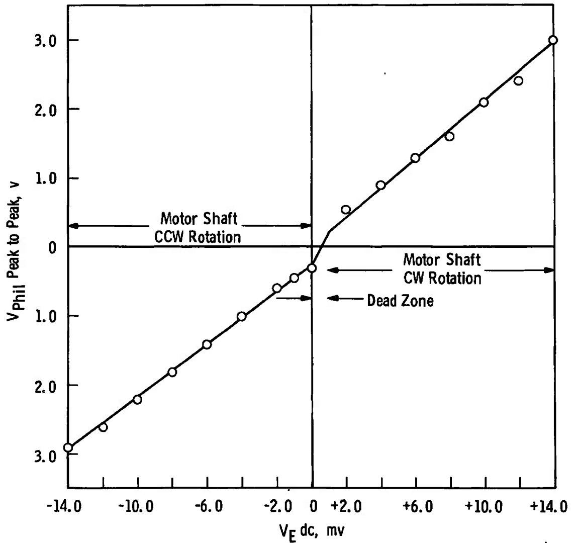
Fig. 7 Error Signal ( V_E ) versus Gas Pumpout Amplifier Input Signal ( V_{\phi} )
