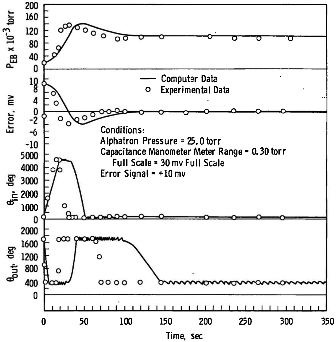
Fig. 14 Transient Response for a Forepressure Set Equal to 1.0 \times 10^{-1} torr
