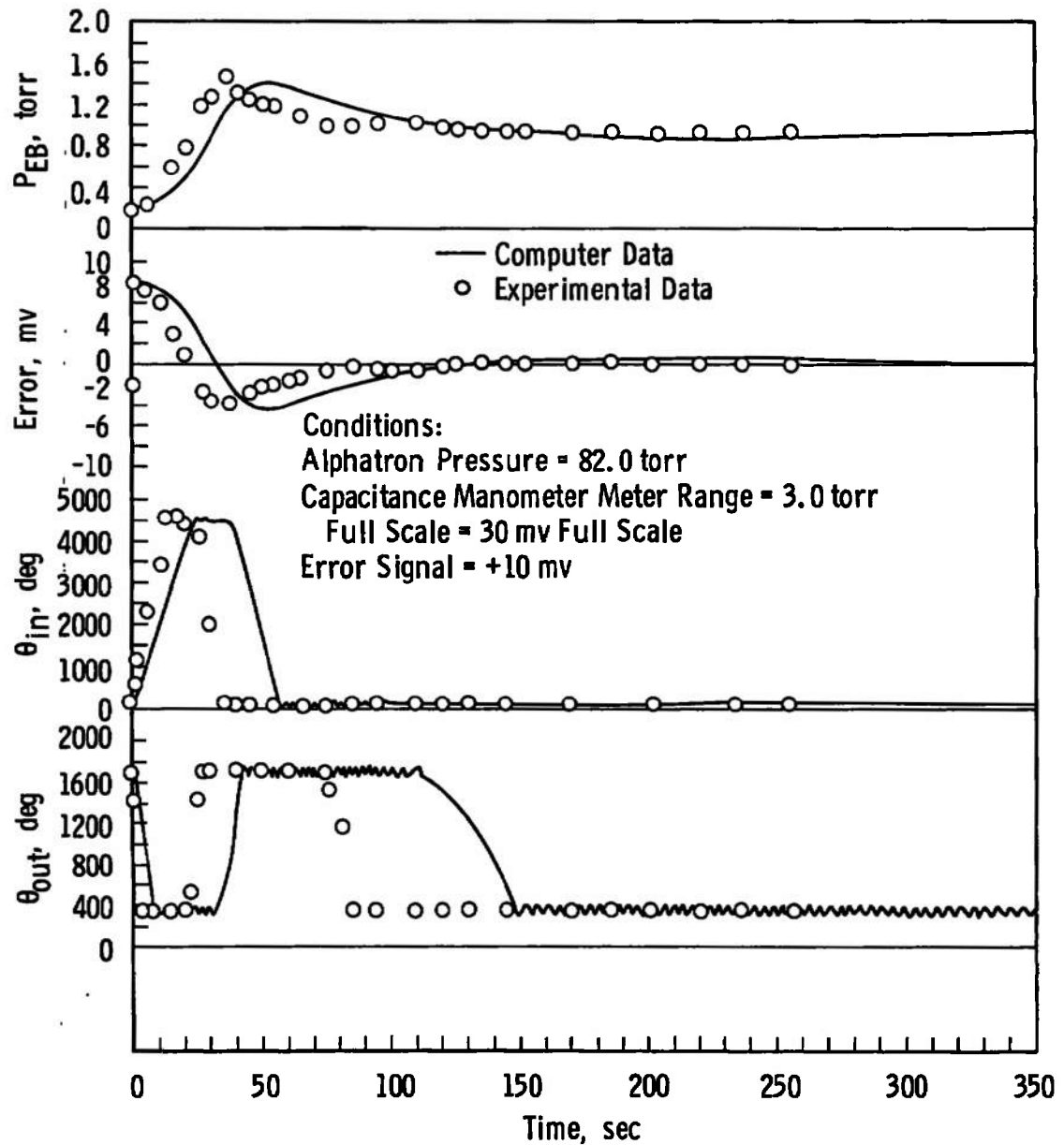
Fig. 17 Transient Response for a Forepressure Set Equal to 1.0 torr
