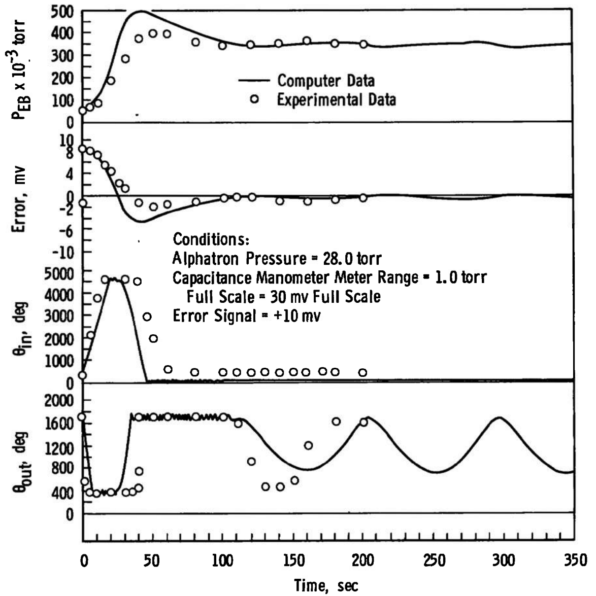
Fig. 15 Transient Response for a Forepressure Set Equal to 3.3 \times 10^{-1} torr
