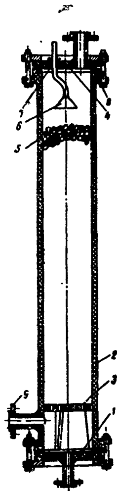
Fig. 5. Faolite column. 1 - bottom; 2 - sheet-steel cylinder; 3 - grat; 4 - lid; 5 - ring fitting; 6 - pipe with funnel; 7 - plug; 8 - flange of sheet-steel cylinder, 9 - connecting pipe flange.
